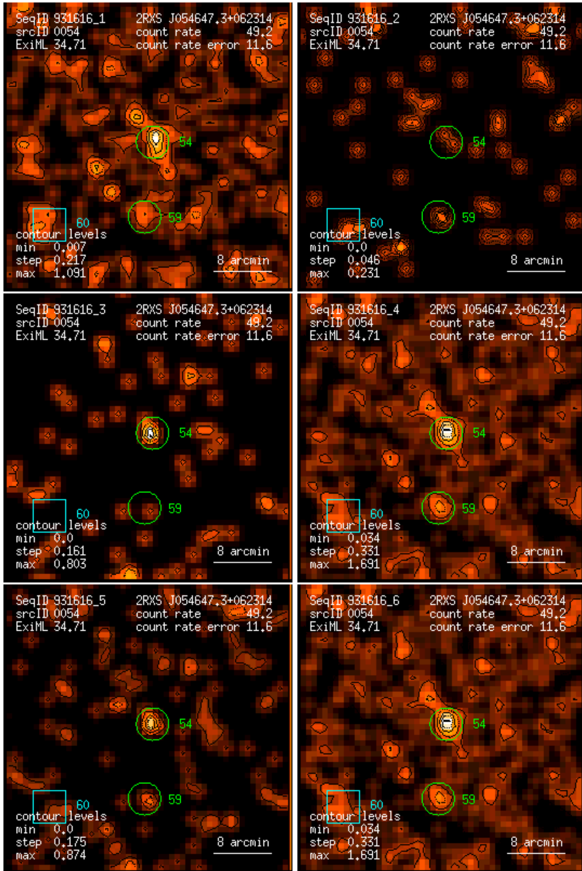
Figure 54: RASS 931616: detection 0054: band rate images, Gaussian filter: (1) PSPC channels 11 – 41, (2) 52 – 90, (3) 91 – 201, (4) 11 – 235, (5) 52 – 201, (6) 11 – 201. Broad band rates in counts/ks. Band rate contour levels in counts/ks/arcmin 2 .
