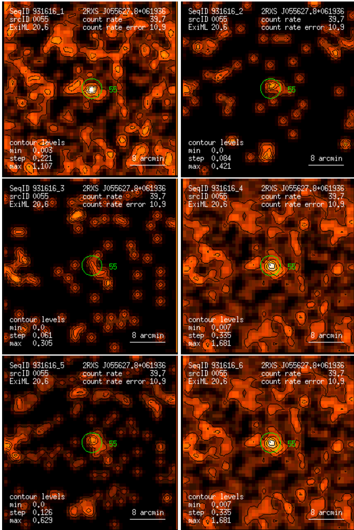
Figure 55: RASS 931616: detection 0055: band rate images, Gaussian filter: (1) PSPC channels 11 – 41, (2) 52 – 90, (3) 91 – 201, (4) 11 – 235, (5) 52 – 201, (6) 11 – 201. Broad band rates in counts/ks. Band rate contour levels in counts/ks/arcmin 2 .
