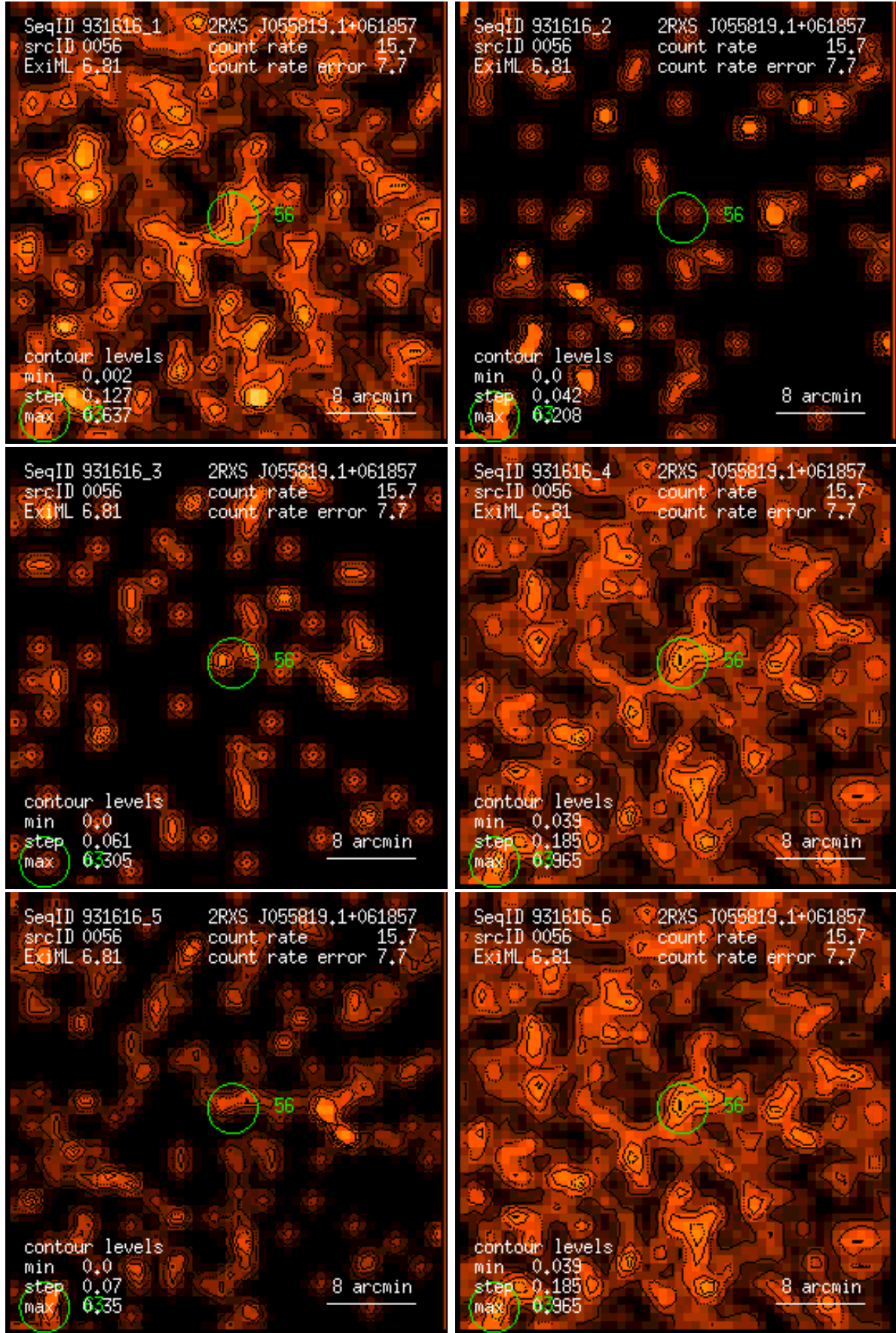
Figure 56: RASS 931616: detection 0056: band rate images, Gaussian filter: (1) PSPC channels 11 – 41, (2) 52 – 90, (3) 91 – 201, (4) 11 – 235, (5) 52 – 201, (6) 11 – 201. Broad band rates in counts/ks. Band rate contour levels in counts/ks/arcmin 2 .
