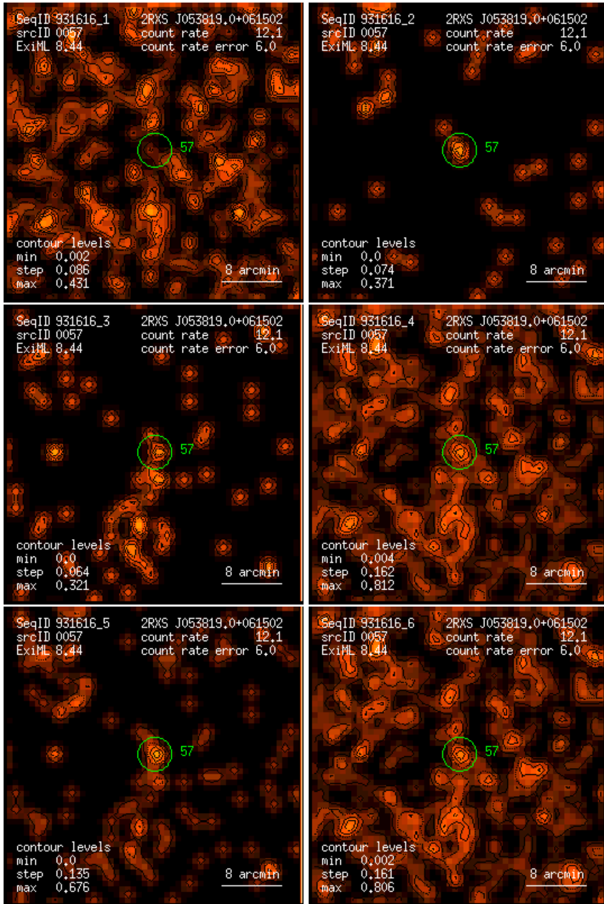
Figure 57: RASS 931616: detection 0057: band rate images, Gaussian filter: (1) PSPC channels 11 – 41, (2) 52 – 90, (3) 91 – 201, (4) 11 – 235, (5) 52 – 201, (6) 11 – 201. Broad band rates in counts/ks. Band rate contour levels in counts/ks/arcmin 2 .
