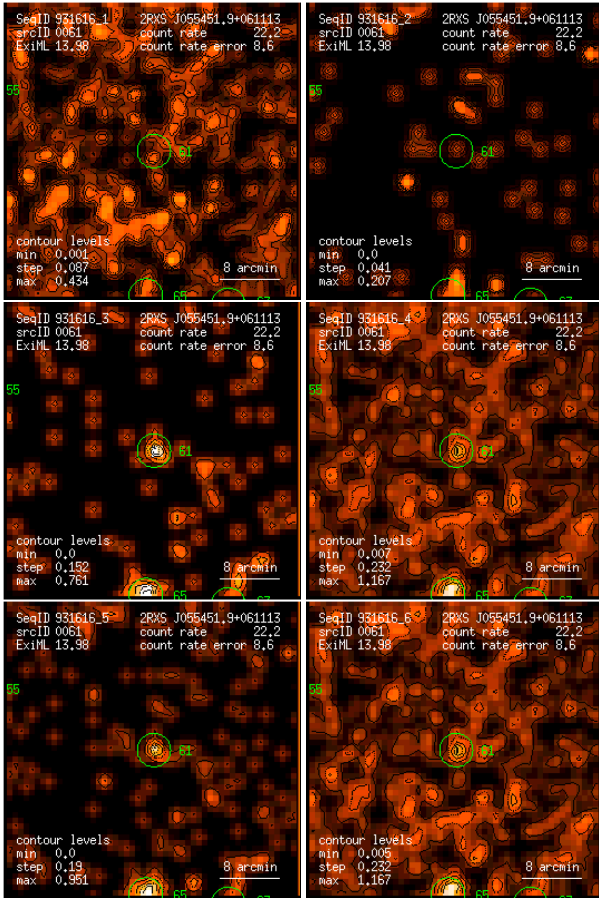
Figure 61: RASS 931616: detection 0061: band rate images, Gaussian filter: (1) PSPC channels 11 – 41, (2) 52 – 90, (3) 91 – 201, (4) 11 – 235, (5) 52 – 201, (6) 11 – 201. Broad band rates in counts/ks. Band rate contour levels in counts/ks/arcmin 2 .
