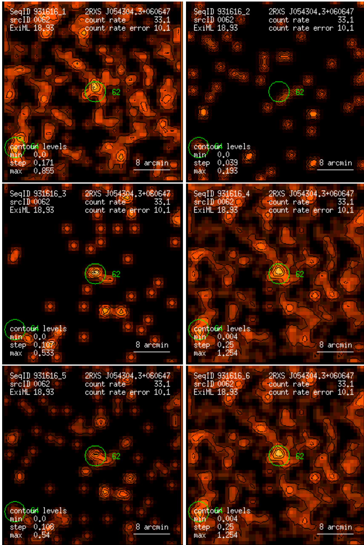
Figure 62: RASS 931616: detection 0062: band rate images, Gaussian filter: (1) PSPC channels 11 – 41, (2) 52 – 90, (3) 91 – 201, (4) 11 – 235, (5) 52 – 201, (6) 11 – 201. Broad band rates in counts/ks. Band rate contour levels in counts/ks/arcmin 2 .
