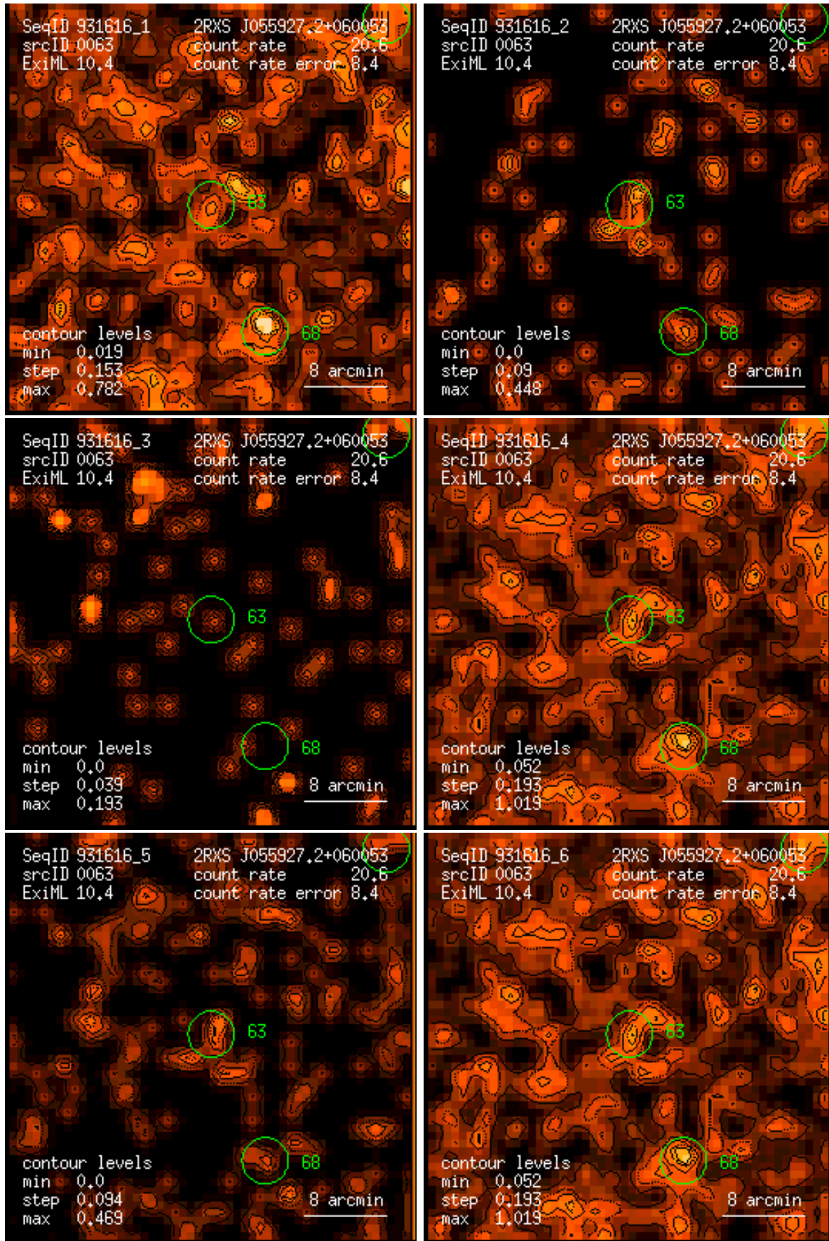
Figure 63: RASS 931616: detection 0063: band rate images, Gaussian filter: (1) PSPC channels 11 – 41, (2) 52 – 90, (3) 91 – 201, (4) 11 – 235, (5) 52 – 201, (6) 11 – 201. Broad band rates in counts/ks. Band rate contour levels in counts/ks/arcmin 2 .
