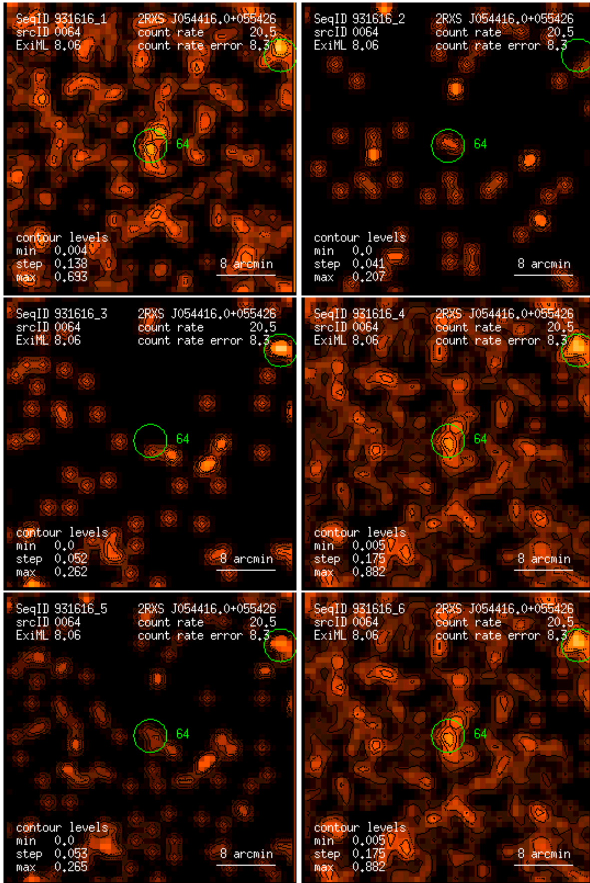
Figure 64: RASS 931616: detection 0064: band rate images, Gaussian filter: (1) PSPC channels 11 – 41, (2) 52 – 90, (3) 91 – 201, (4) 11 – 235, (5) 52 – 201, (6) 11 – 201. Broad band rates in counts/ks. Band rate contour levels in counts/ks/arcmin 2 .
