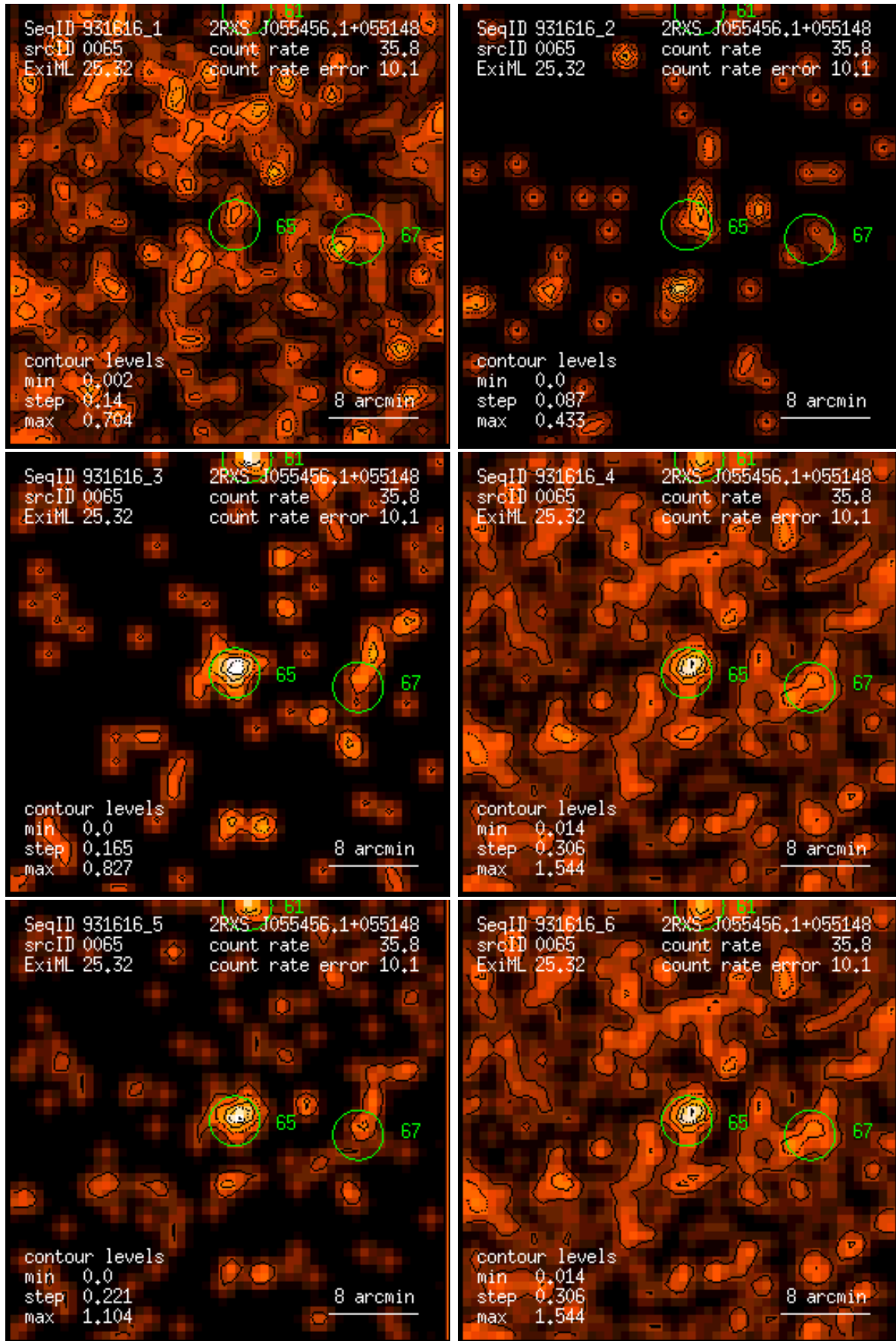
Figure 65: RASS 931616: detection 0065: band rate images, Gaussian filter: (1) PSPC channels 11 – 41, (2) 52 – 90, (3) 91 – 201, (4) 11 – 235, (5) 52 – 201, (6) 11 – 201. Broad band rates in counts/ks. Band rate contour levels in counts/ks/arcmin 2 .
