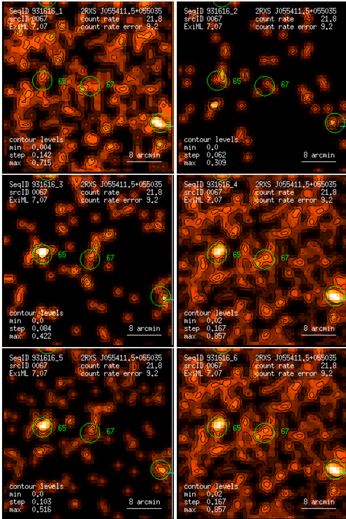
Figure 67: RASS 931616: detection 0067: band rate images, Gaussian filter: (1) PSPC channels 11 – 41, (2) 52 – 90, (3) 91 – 201, (4) 11 – 235, (5) 52 – 201, (6) 11 – 201. Broad band rates in counts/ks. Band rate contour levels in counts/ks/arcmin 2 .
