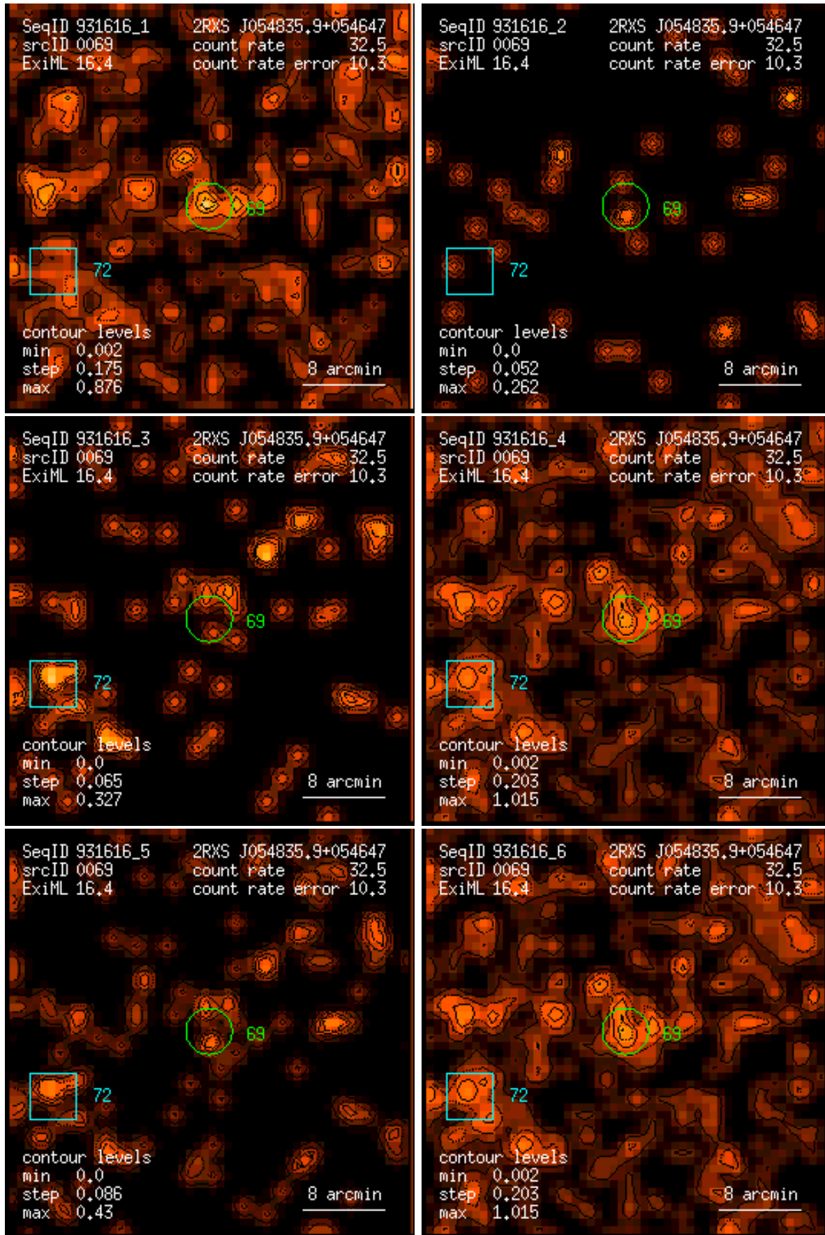
Figure 69: RASS 931616: detection 0069: band rate images, Gaussian filter: (1) PSPC channels 11 – 41, (2) 52 – 90, (3) 91 – 201, (4) 11 – 235, (5) 52 – 201, (6) 11 – 201. Broad band rates in counts/ks. Band rate contour levels in counts/ks/arcmin 2 .
