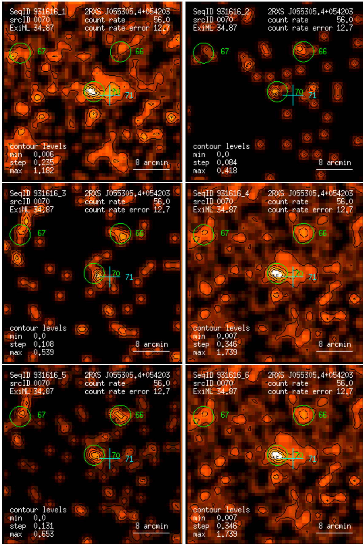
Figure 70: RASS 931616: detection 0070: band rate images, Gaussian filter: (1) PSPC channels 11 – 41, (2) 52 – 90, (3) 91 – 201, (4) 11 – 235, (5) 52 – 201, (6) 11 – 201. Broad band rates in counts/ks. Band rate contour levels in counts/ks/arcmin 2 .
