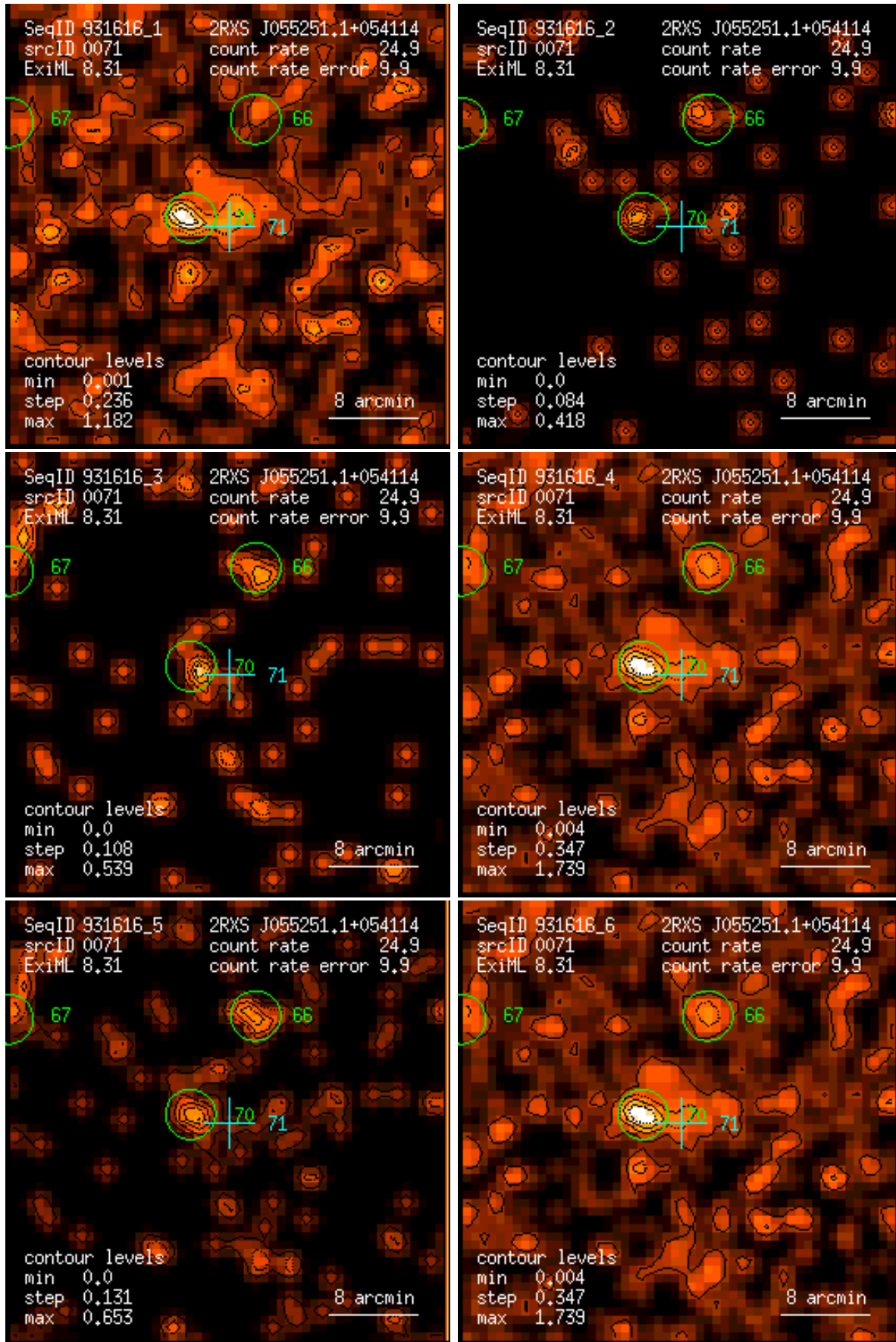
Figure 71: RASS 931616: detection 0071: band rate images, Gaussian filter: (1) PSPC channels 11 – 41, (2) 52 – 90, (3) 91 – 201, (4) 11 – 235, (5) 52 – 201, (6) 11 – 201. Broad band rates in counts/ks. Band rate contour levels in counts/ks/arcmin 2 .
