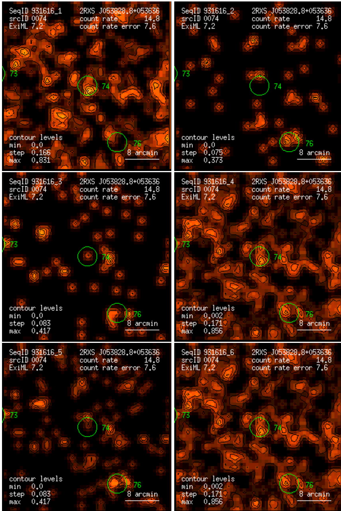
Figure 74: RASS 931616: detection 0074: band rate images, Gaussian filter: (1) PSPC channels 11 – 41, (2) 52 – 90, (3) 91 – 201, (4) 11 – 235, (5) 52 – 201, (6) 11 – 201. Broad band rates in counts/ks. Band rate contour levels in counts/ks/arcmin 2 .
