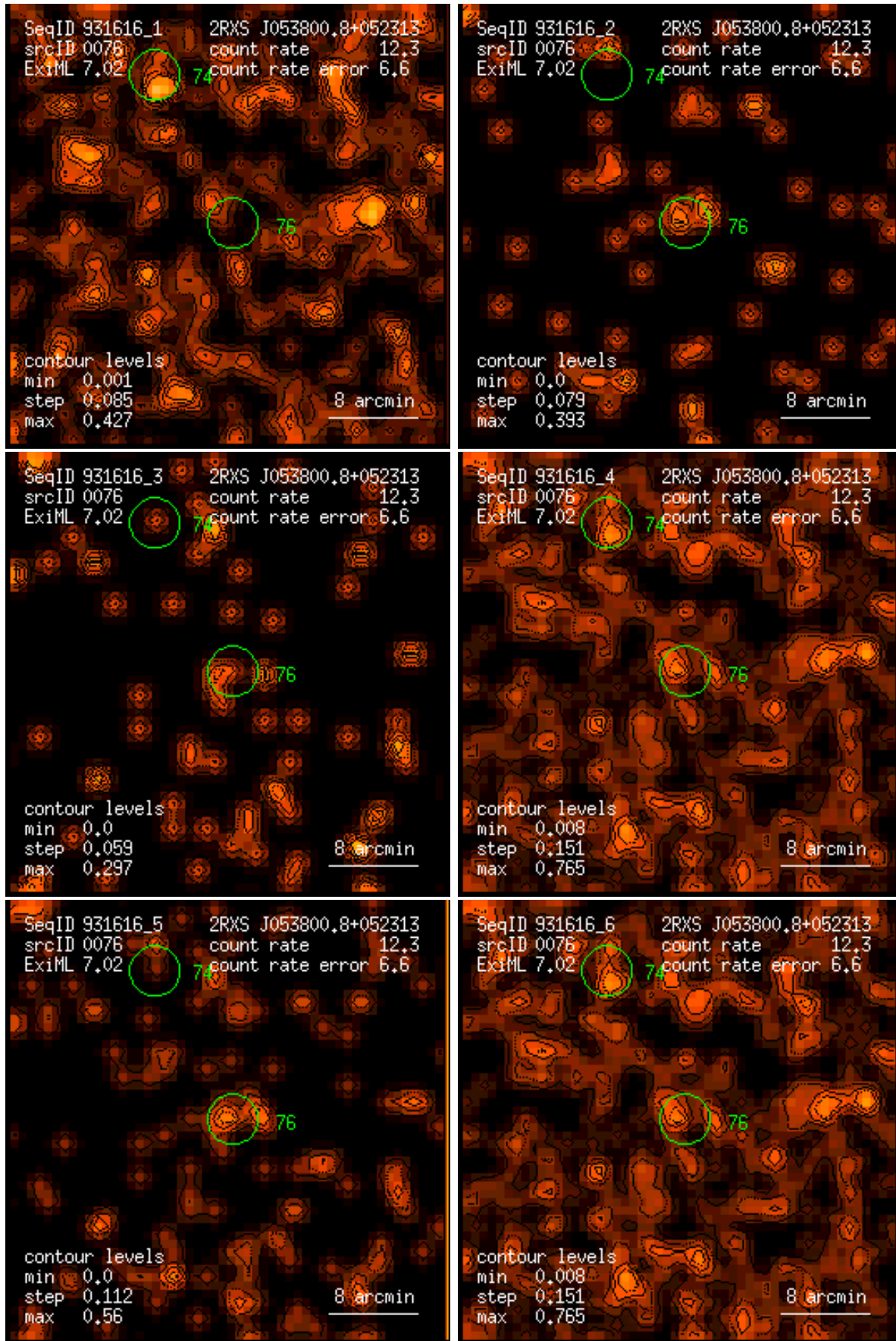
Figure 76: RASS 931616: detection 0076: band rate images, Gaussian filter: (1) PSPC channels 11 – 41, (2) 52 – 90, (3) 91 – 201, (4) 11 – 235, (5) 52 – 201, (6) 11 – 201. Broad band rates in counts/ks. Band rate contour levels in counts/ks/arcmin 2 .
