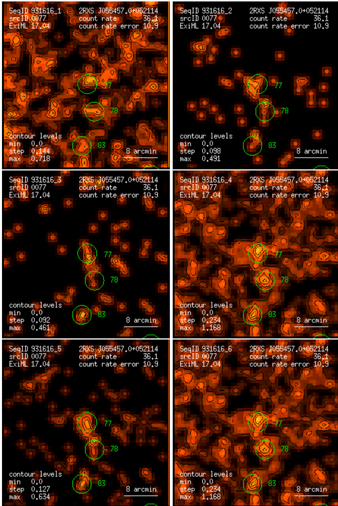
Figure 77: RASS 931616: detection 0077: band rate images, Gaussian filter: (1) PSPC channels 11 – 41, (2) 52 – 90, (3) 91 – 201, (4) 11 – 235, (5) 52 – 201, (6) 11 – 201. Broad band rates in counts/ks. Band rate contour levels in counts/ks/arcmin 2 .
