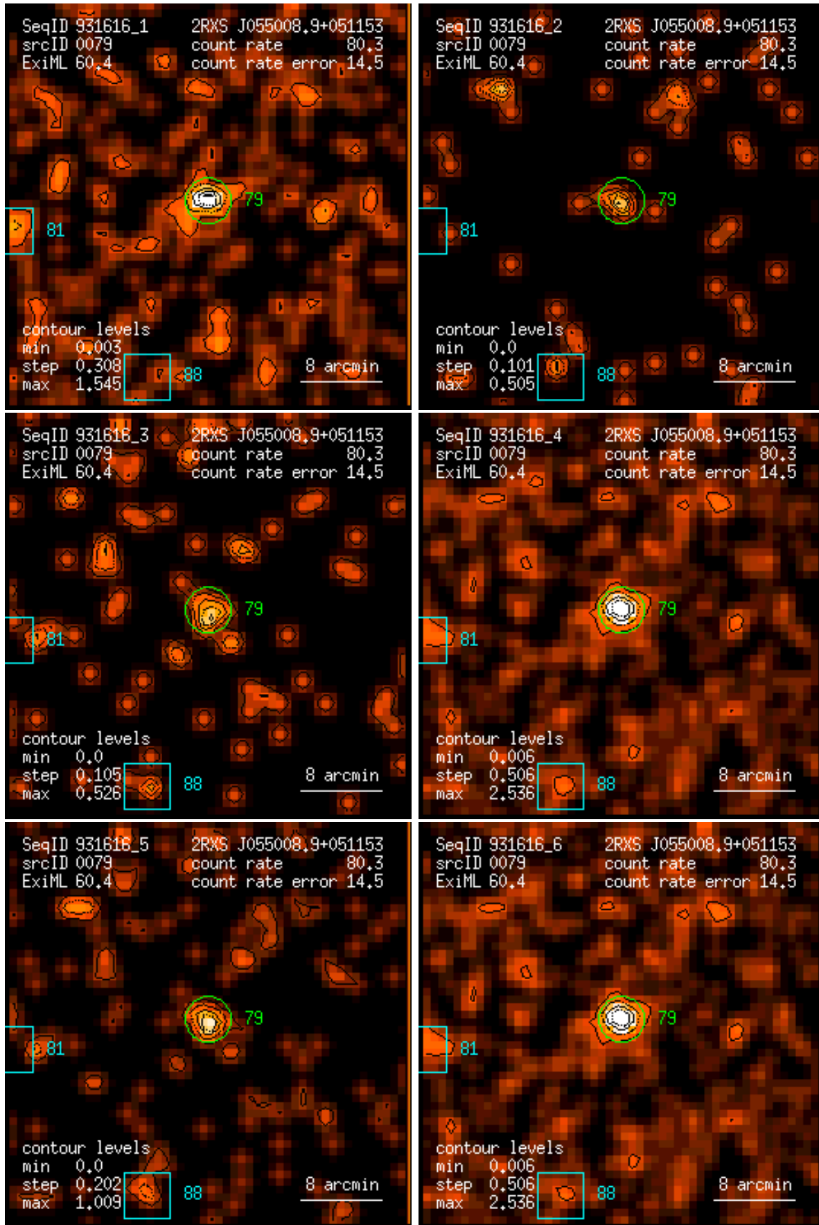
Figure 79: RASS 931616: detection 0079: band rate images, Gaussian filter: (1) PSPC channels 11 – 41, (2) 52 – 90, (3) 91 – 201, (4) 11 – 235, (5) 52 – 201, (6) 11 – 201. Broad band rates in counts/ks. Band rate contour levels in counts/ks/arcmin 2 .
