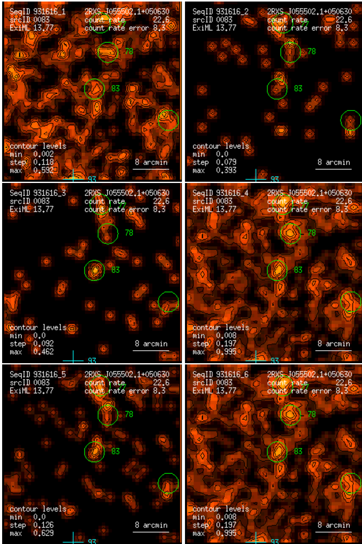
Figure 83: RASS 931616: detection 0083: band rate images, Gaussian filter: (1) PSPC channels 11 – 41, (2) 52 – 90, (3) 91 – 201, (4) 11 – 235, (5) 52 – 201, (6) 11 – 201. Broad band rates in counts/ks. Band rate contour levels in counts/ks/arcmin 2 .
