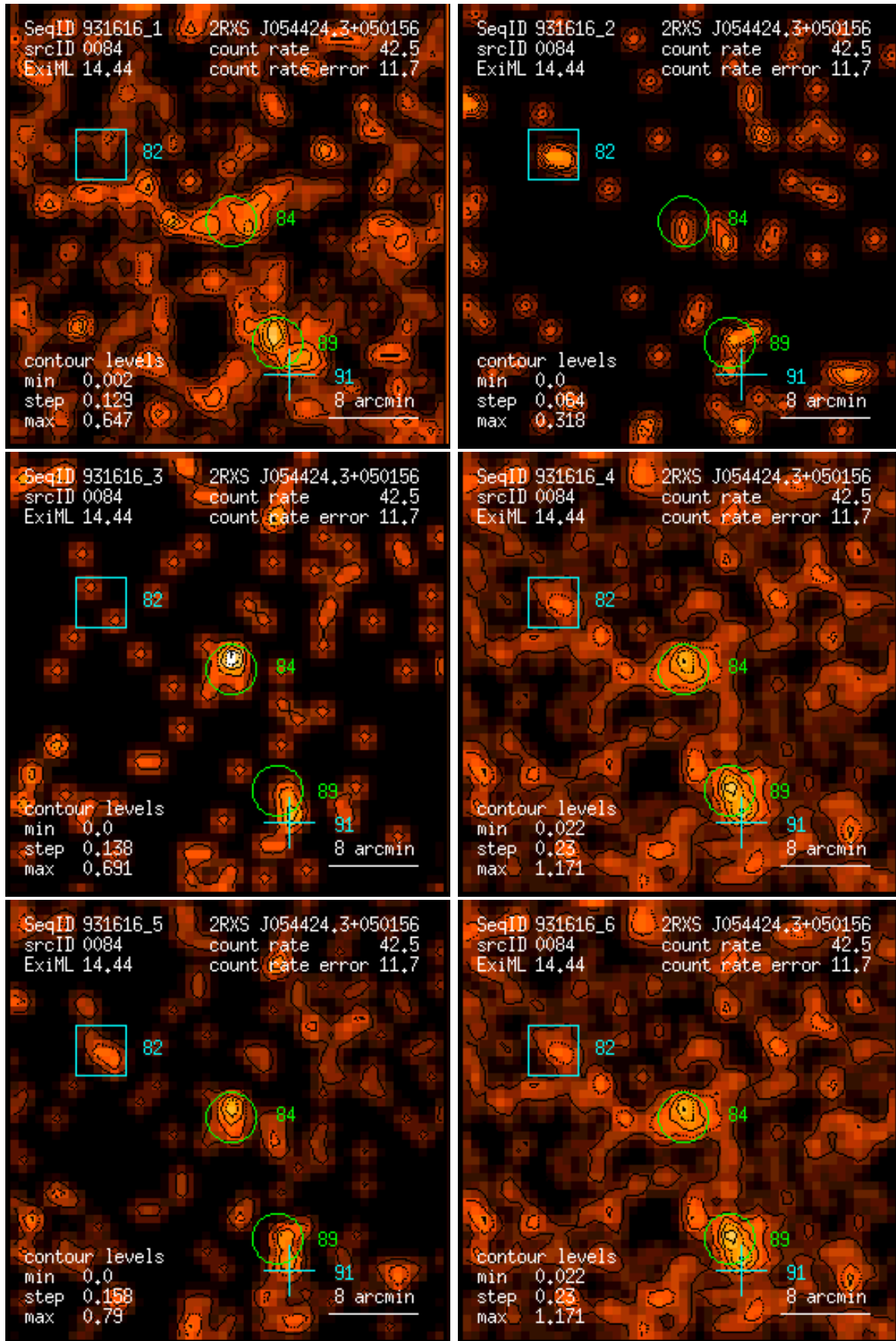
Figure 84: RASS 931616: detection 0084: band rate images, Gaussian filter: (1) PSPC channels 11 – 41, (2) 52 – 90, (3) 91 – 201, (4) 11 – 235, (5) 52 – 201, (6) 11 – 201. Broad band rates in counts/ks. Band rate contour levels in counts/ks/arcmin 2 .
