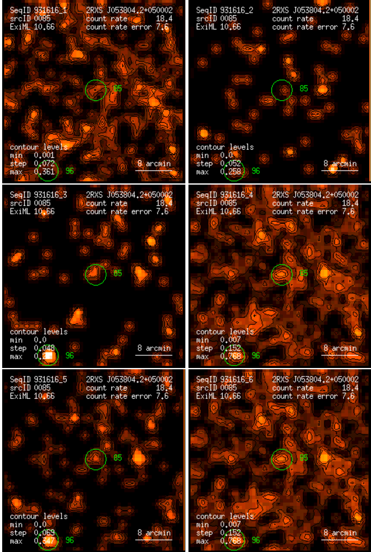
Figure 85: RASS 931616: detection 0085: band rate images, Gaussian filter: (1) PSPC channels 11 – 41, (2) 52 – 90, (3) 91 – 201, (4) 11 – 235, (5) 52 – 201, (6) 11 – 201. Broad band rates in counts/ks. Band rate contour levels in counts/ks/arcmin 2 .
