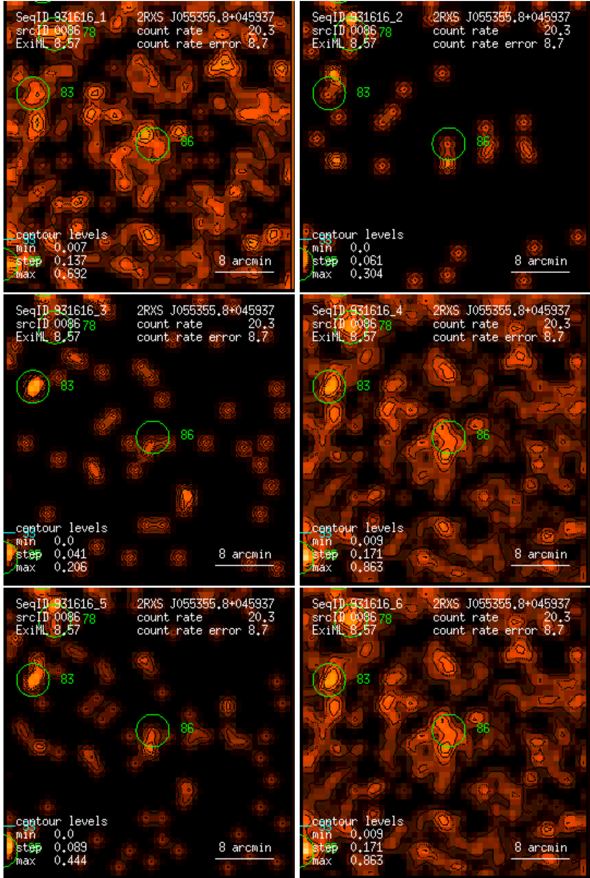
Figure 86: RASS 931616: detection 0086: band rate images, Gaussian filter: (1) PSPC channels 11 – 41, (2) 52 – 90, (3) 91 – 201, (4) 11 – 235, (5) 52 – 201, (6) 11 – 201. Broad band rates in counts/ks. Band rate contour levels in counts/ks/arcmin 2 .
