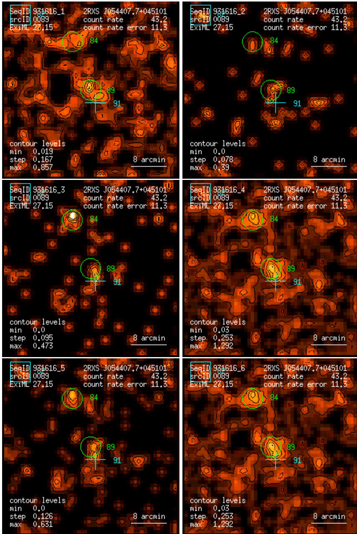
Figure 89: RASS 931616: detection 0089: band rate images, Gaussian filter: (1) PSPC channels 11 – 41, (2) 52 – 90, (3) 91 – 201, (4) 11 – 235, (5) 52 – 201, (6) 11 – 201. Broad band rates in counts/ks. Band rate contour levels in counts/ks/arcmin 2 .
