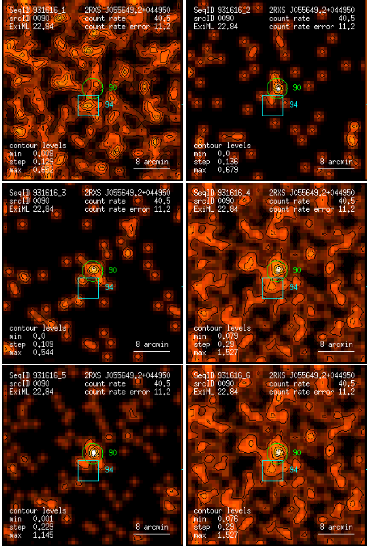
Figure 90: RASS 931616: detection 0090: band rate images, Gaussian filter: (1) PSPC channels 11 – 41, (2) 52 – 90, (3) 91 – 201, (4) 11 – 235, (5) 52 – 201, (6) 11 – 201. Broad band rates in counts/ks. Band rate contour levels in counts/ks/arcmin 2 .
