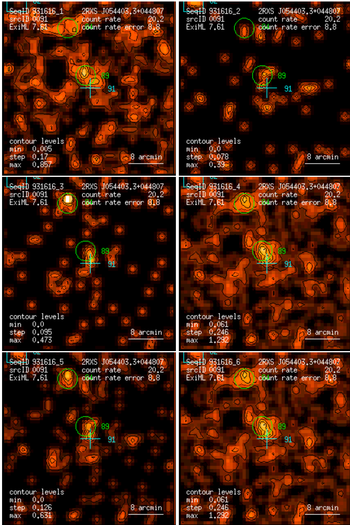
Figure 91: RASS 931616: detection 0091: band rate images, Gaussian filter: (1) PSPC channels 11 – 41, (2) 52 – 90, (3) 91 – 201, (4) 11 – 235, (5) 52 – 201, (6) 11 – 201. Broad band rates in counts/ks. Band rate contour levels in counts/ks/arcmin 2 .
