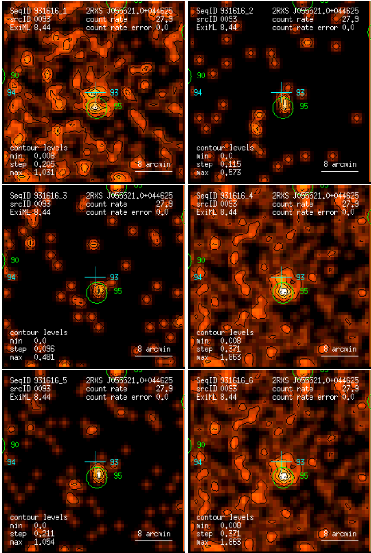
Figure 93: RASS 931616: detection 0093: band rate images, Gaussian filter: (1) PSPC channels 11 – 41, (2) 52 – 90, (3) 91 – 201, (4) 11 – 235, (5) 52 – 201, (6) 11 – 201. Broad band rates in counts/ks. Band rate contour levels in counts/ks/arcmin 2 .
