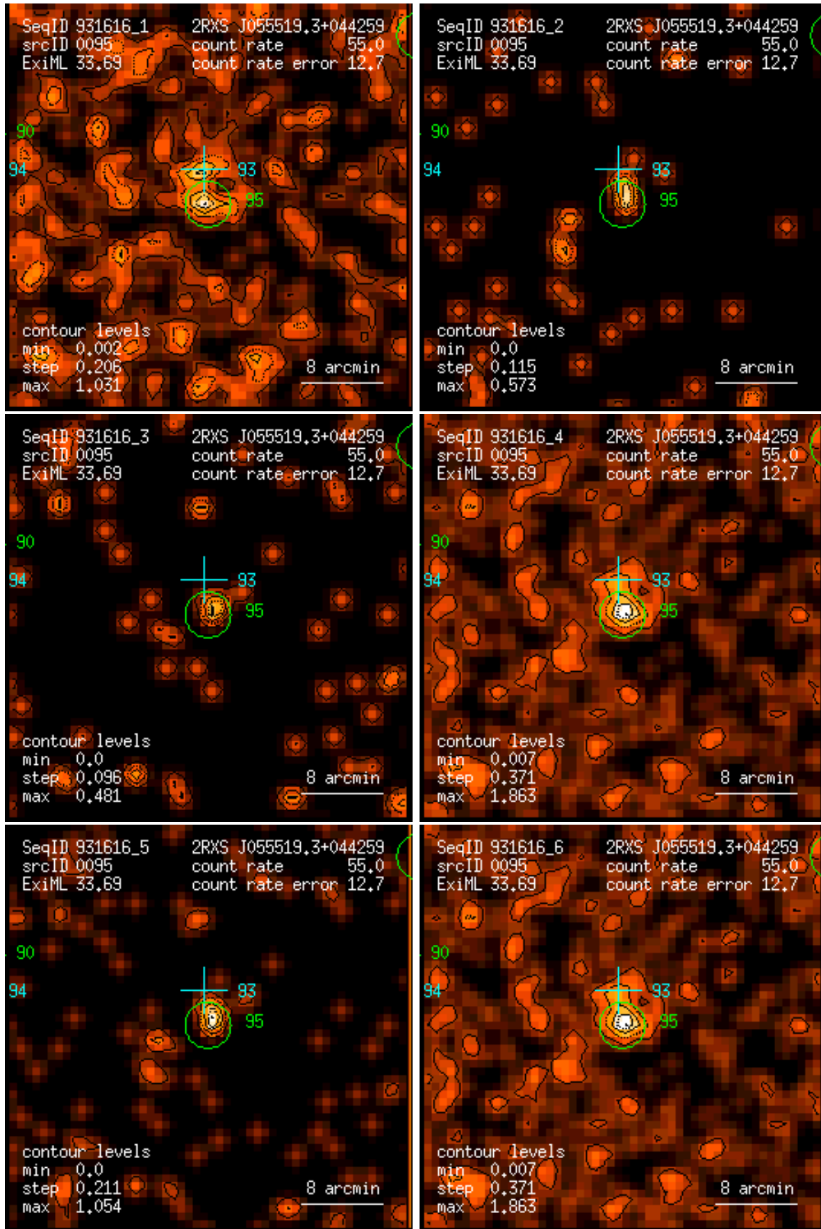
Figure 95: RASS 931616: detection 0095: band rate images, Gaussian filter: (1) PSPC channels 11 – 41, (2) 52 – 90, (3) 91 – 201, (4) 11 – 235, (5) 52 – 201, (6) 11 – 201. Broad band rates in counts/ks. Band rate contour levels in counts/ks/arcmin 2 .
