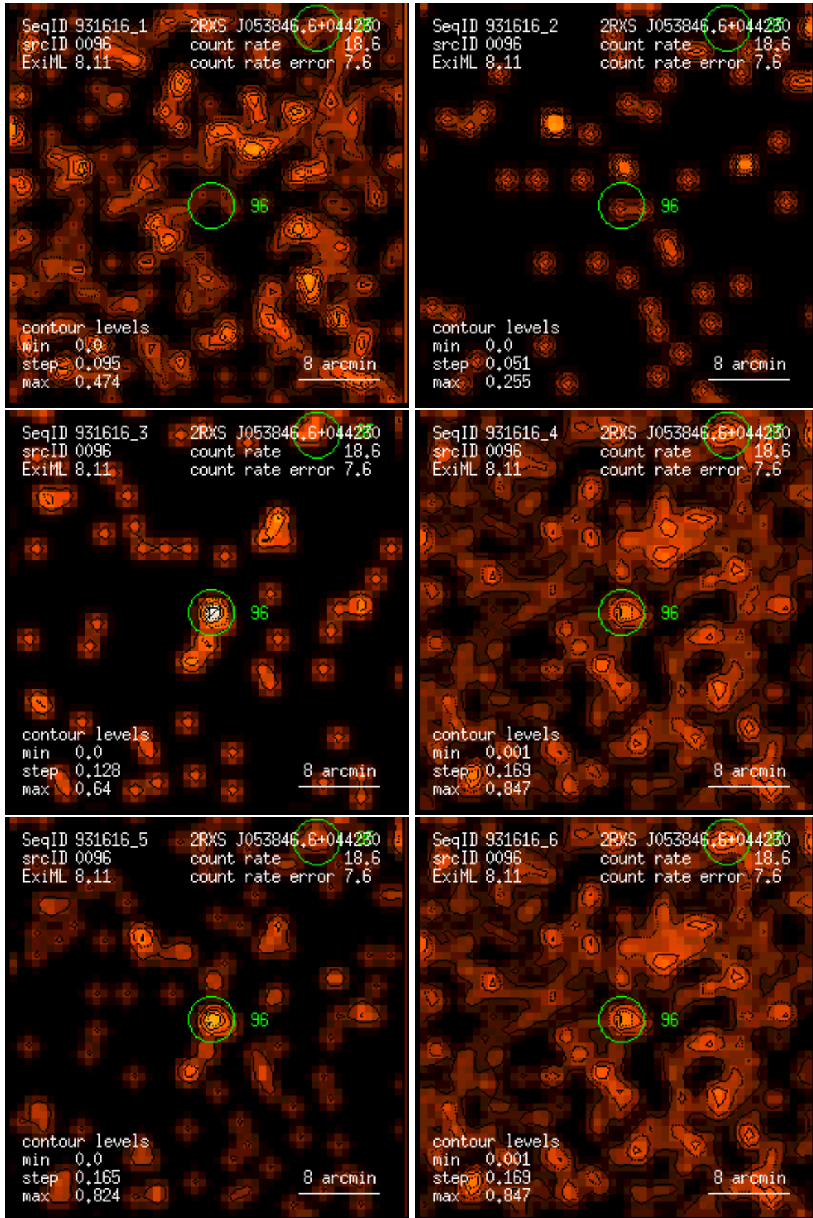
Figure 96: RASS 931616: detection 0096: band rate images, Gaussian filter: (1) PSPC channels 11 – 41, (2) 52 – 90, (3) 91 – 201, (4) 11 – 235, (5) 52 – 201, (6) 11 – 201. Broad band rates in counts/ks. Band rate contour levels in counts/ks/arcmin 2 .
