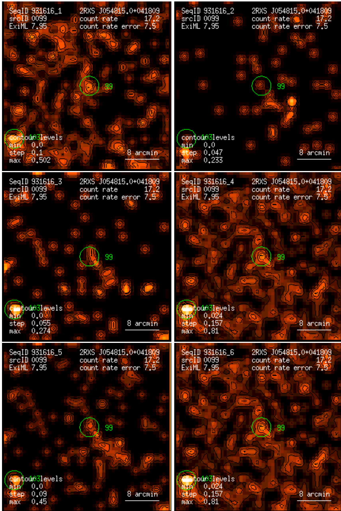
Figure 99: RASS 931616: detection 0099: band rate images, Gaussian filter: (1) PSPC channels 11 – 41, (2) 52 – 90, (3) 91 – 201, (4) 11 – 235, (5) 52 – 201, (6) 11 – 201. Broad band rates in counts/ks. Band rate contour levels in counts/ks/arcmin 2 .
