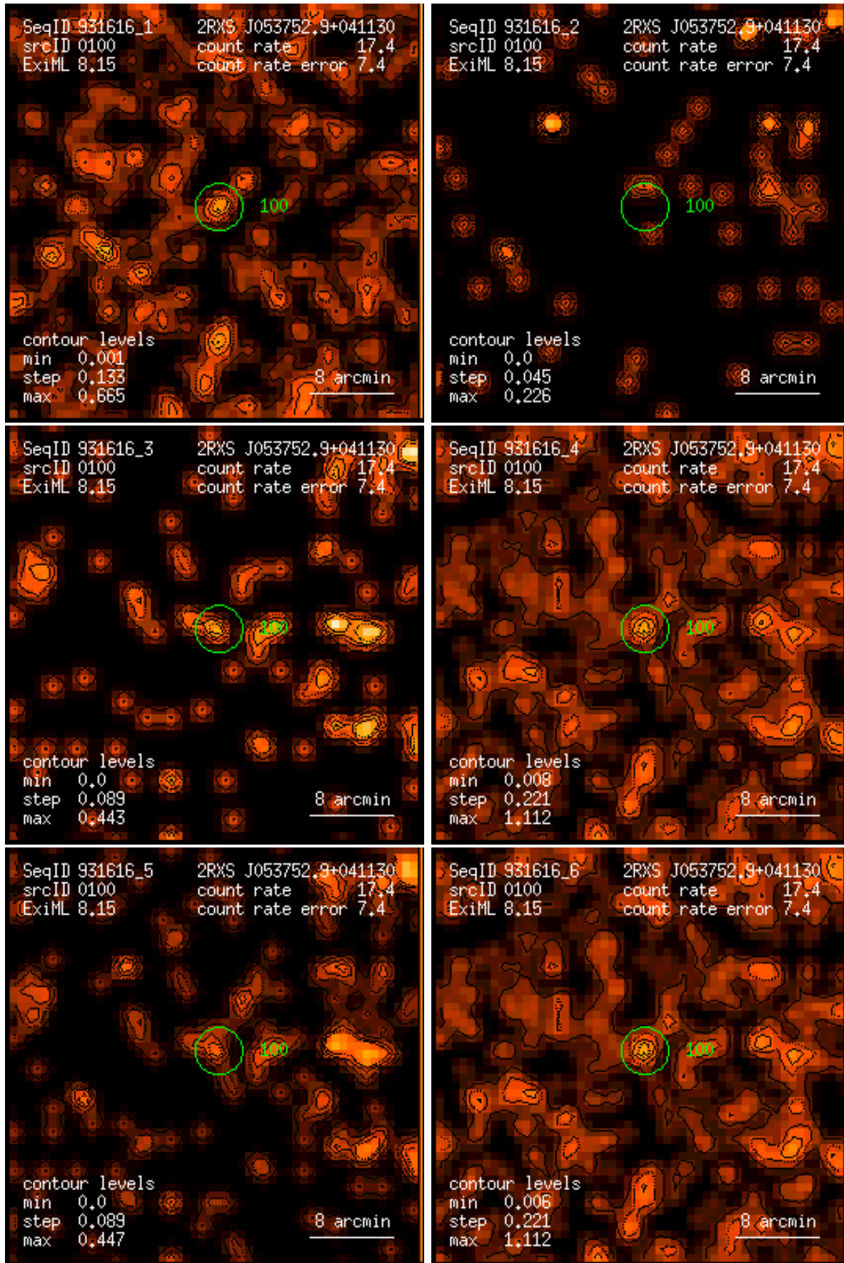
Figure 100: RASS 931616: detection 0100: band rate images, Gaussian filter: (1) PSPC channels 11 – 41, (2) 52 – 90, (3) 91 – 201, (4) 11 – 235, (5) 52 – 201, (6) 11 – 201. Broad band rates in counts/ks. Band rate contour levels in counts/ks/arcmin 2 .
