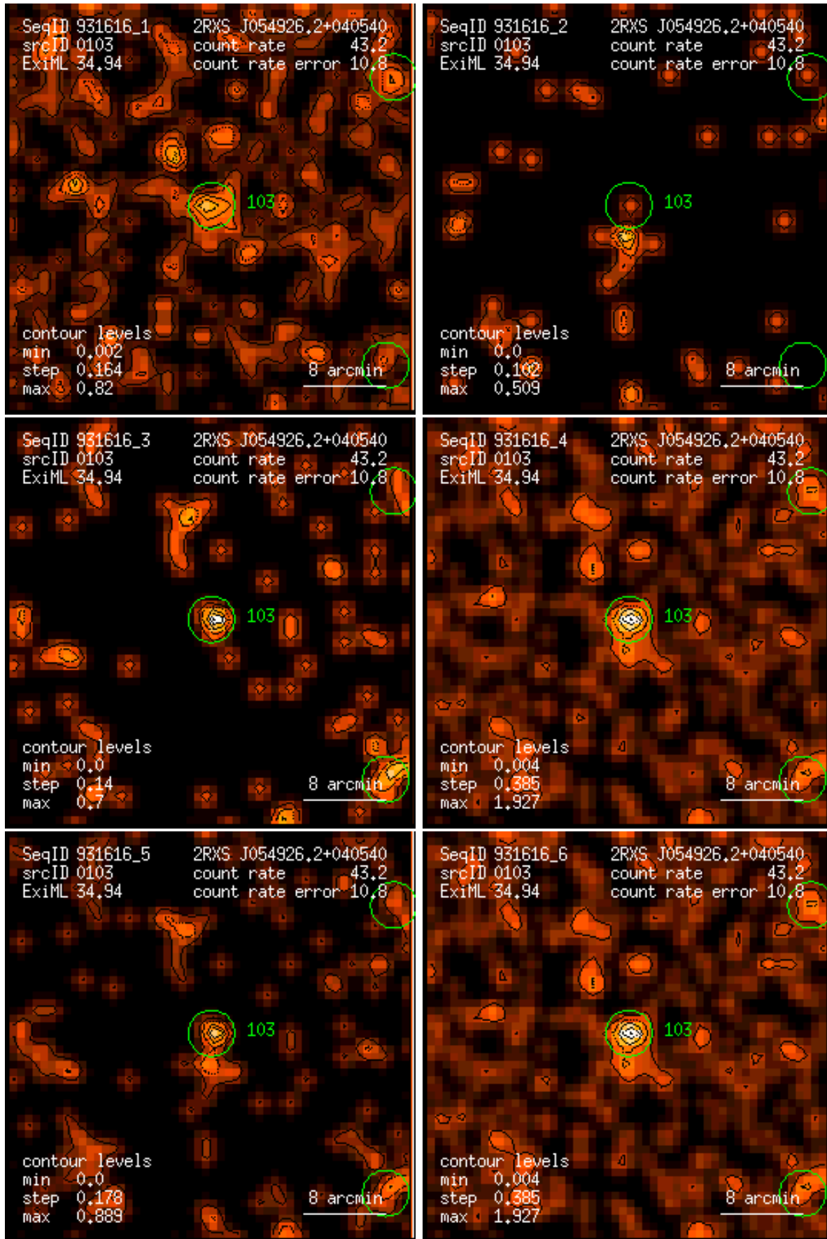
Figure 103: RASS 931616: detection 0103: band rate images, Gaussian filter: (1) PSPC channels 11 – 41, (2) 52 – 90, (3) 91 – 201, (4) 11 – 235, (5) 52 – 201, (6) 11 – 201. Broad band rates in counts/ks. Band rate contour levels in counts/ks/arcmin 2 .
