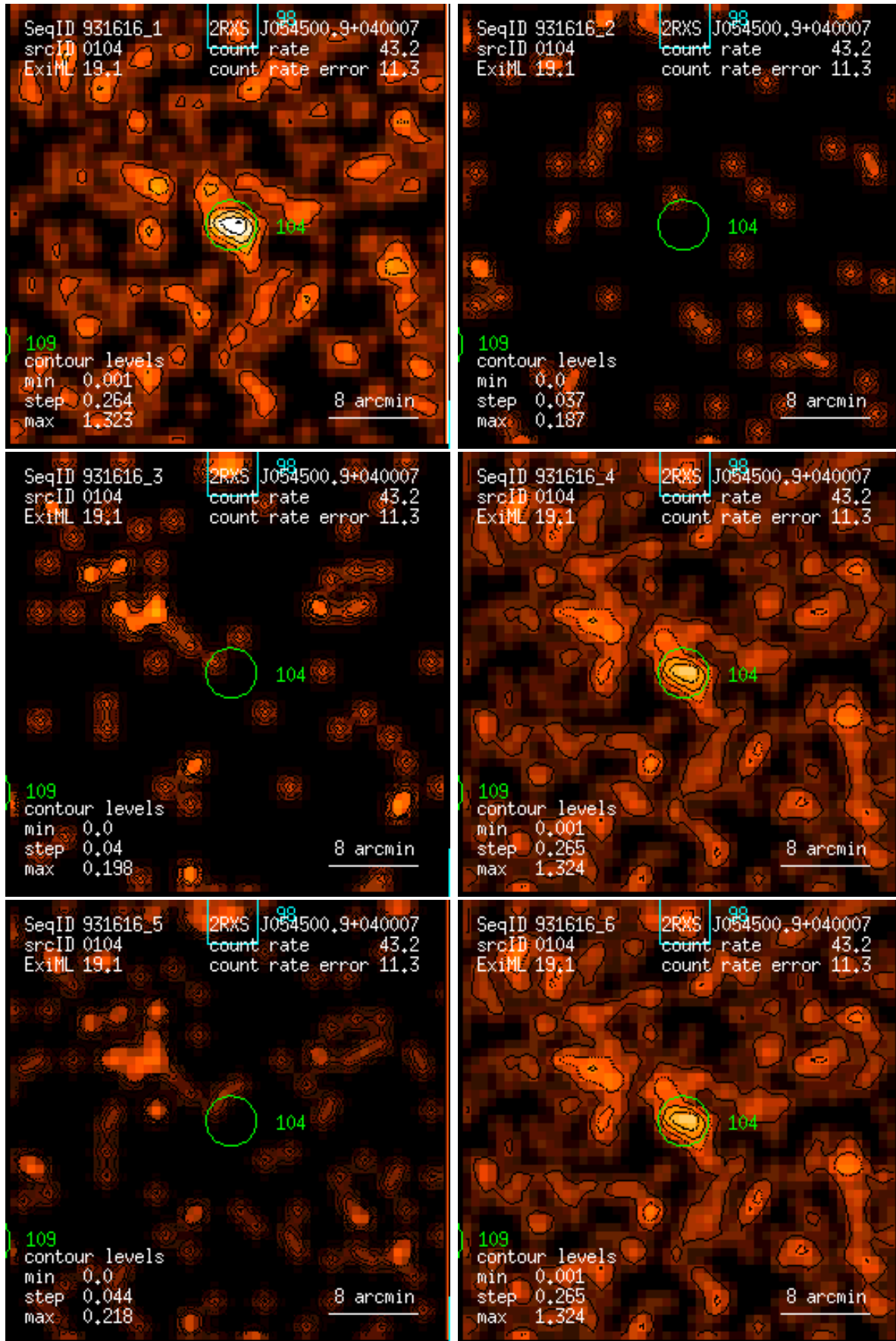
Figure 104: RASS 931616: detection 0104: band rate images, Gaussian filter: (1) PSPC channels 11 – 41, (2) 52 – 90, (3) 91 – 201, (4) 11 – 235, (5) 52 – 201, (6) 11 – 201. Broad band rates in counts/ks. Band rate contour levels in counts/ks/arcmin 2 .
