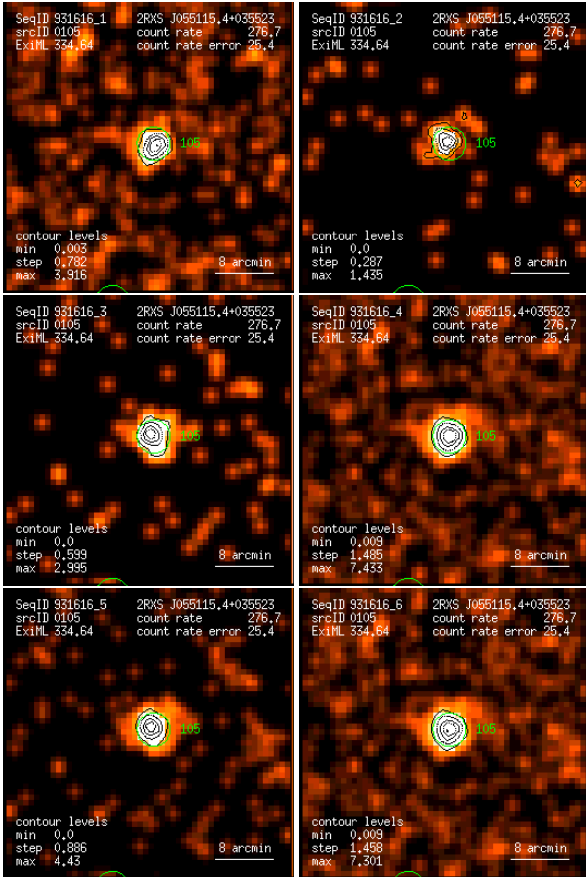
Figure 105: RASS 931616: detection 0105: band rate images, Gaussian filter: (1) PSPC channels 11 – 41, (2) 52 – 90, (3) 91 – 201, (4) 11 – 235, (5) 52 – 201, (6) 11 – 201. Broad band rates in counts/ks. Band rate contour levels in counts/ks/arcmin 2 .
