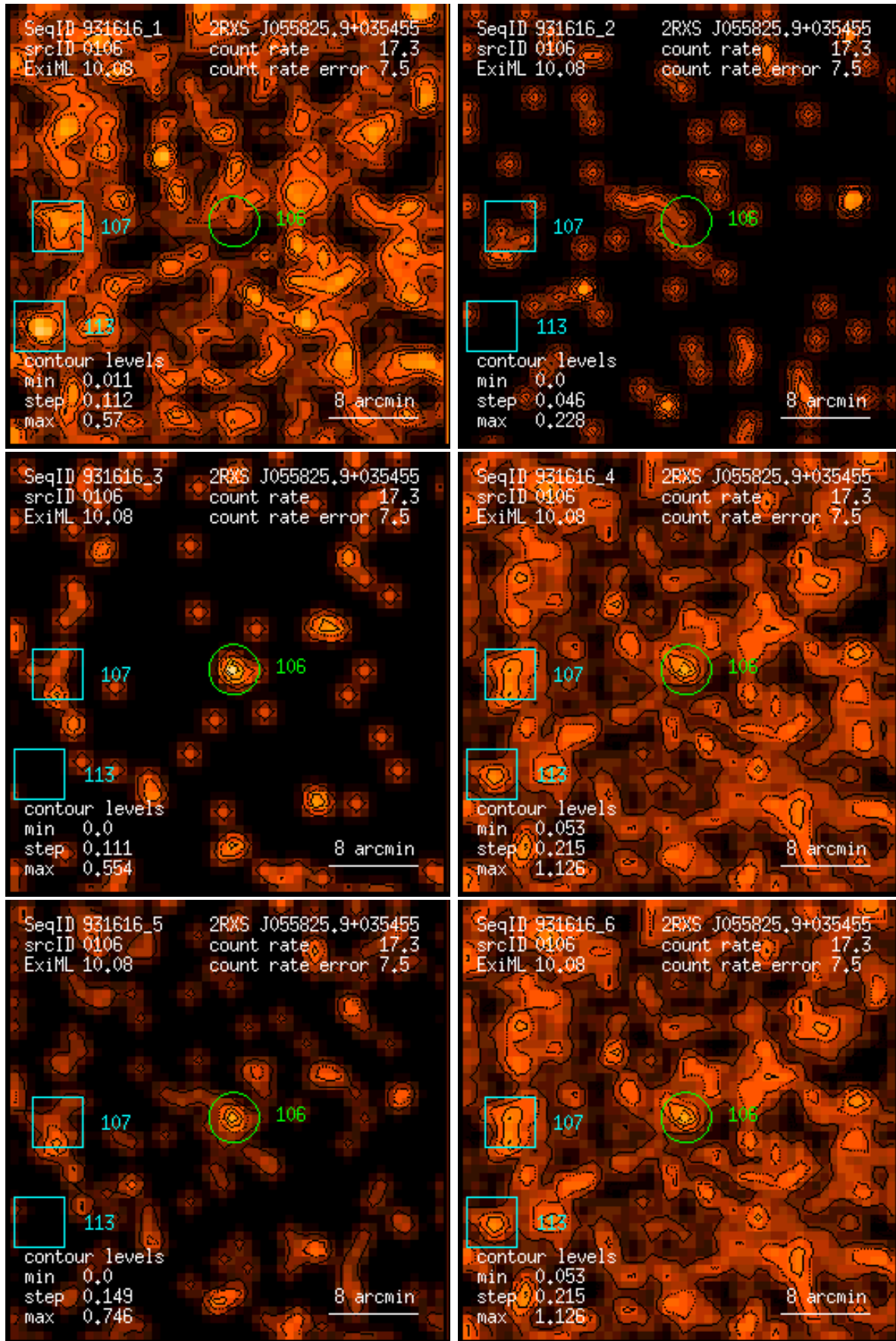
Figure 106: RASS 931616: detection 0106: band rate images, Gaussian filter: (1) PSPC channels 11 – 41, (2) 52 – 90, (3) 91 – 201, (4) 11 – 235, (5) 52 – 201, (6) 11 – 201. Broad band rates in counts/ks. Band rate contour levels in counts/ks/arcmin 2 .
