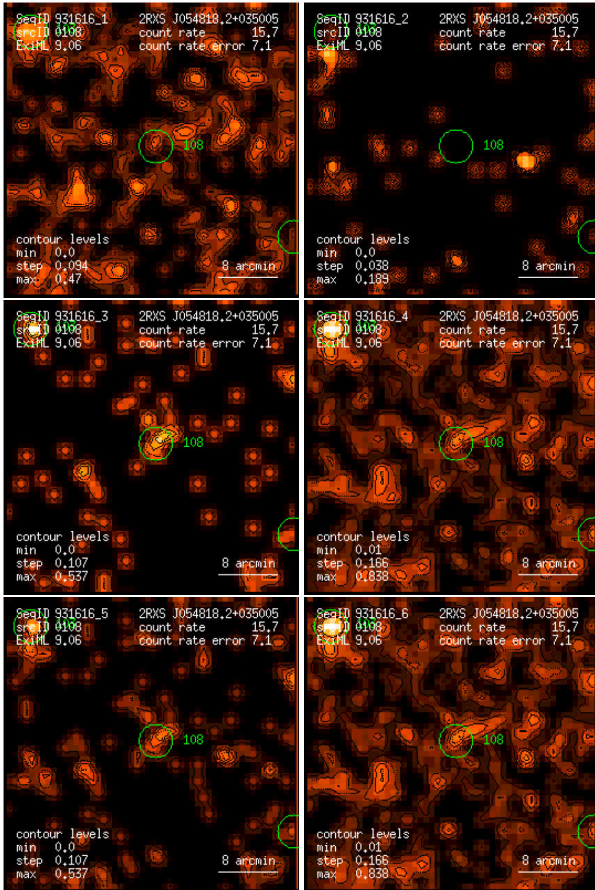
Figure 108: RASS 931616: detection 0108: band rate images, Gaussian filter: (1) PSPC channels 11 – 41, (2) 52 – 90, (3) 91 – 201, (4) 11 – 235, (5) 52 – 201, (6) 11 – 201. Broad band rates in counts/ks. Band rate contour levels in counts/ks/arcmin 2 .
