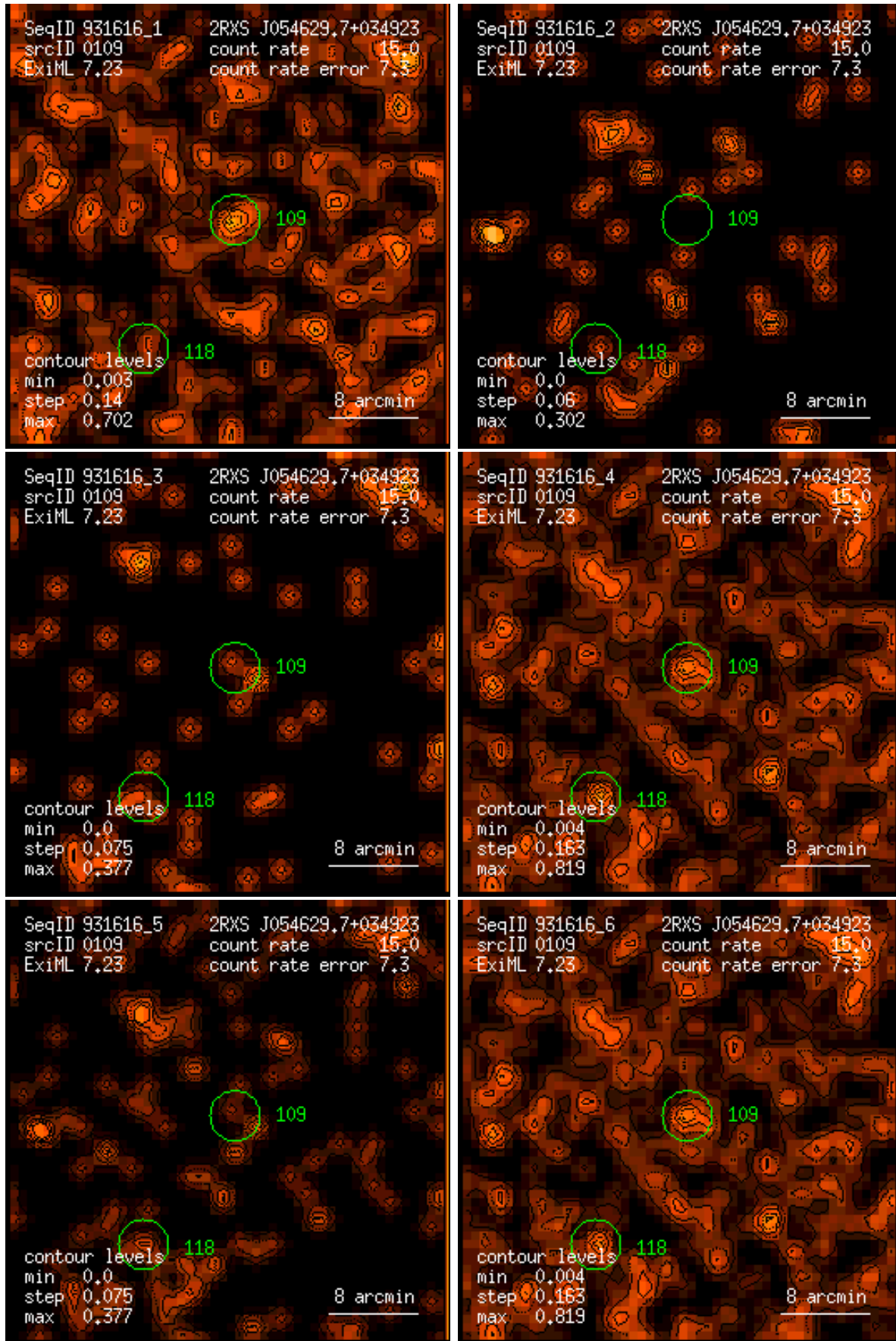
Figure 109: RASS 931616: detection 0109: band rate images, Gaussian filter: (1) PSPC channels 11 – 41, (2) 52 – 90, (3) 91 – 201, (4) 11 – 235, (5) 52 – 201, (6) 11 – 201. Broad band rates in counts/ks. Band rate contour levels in counts/ks/arcmin 2 .
