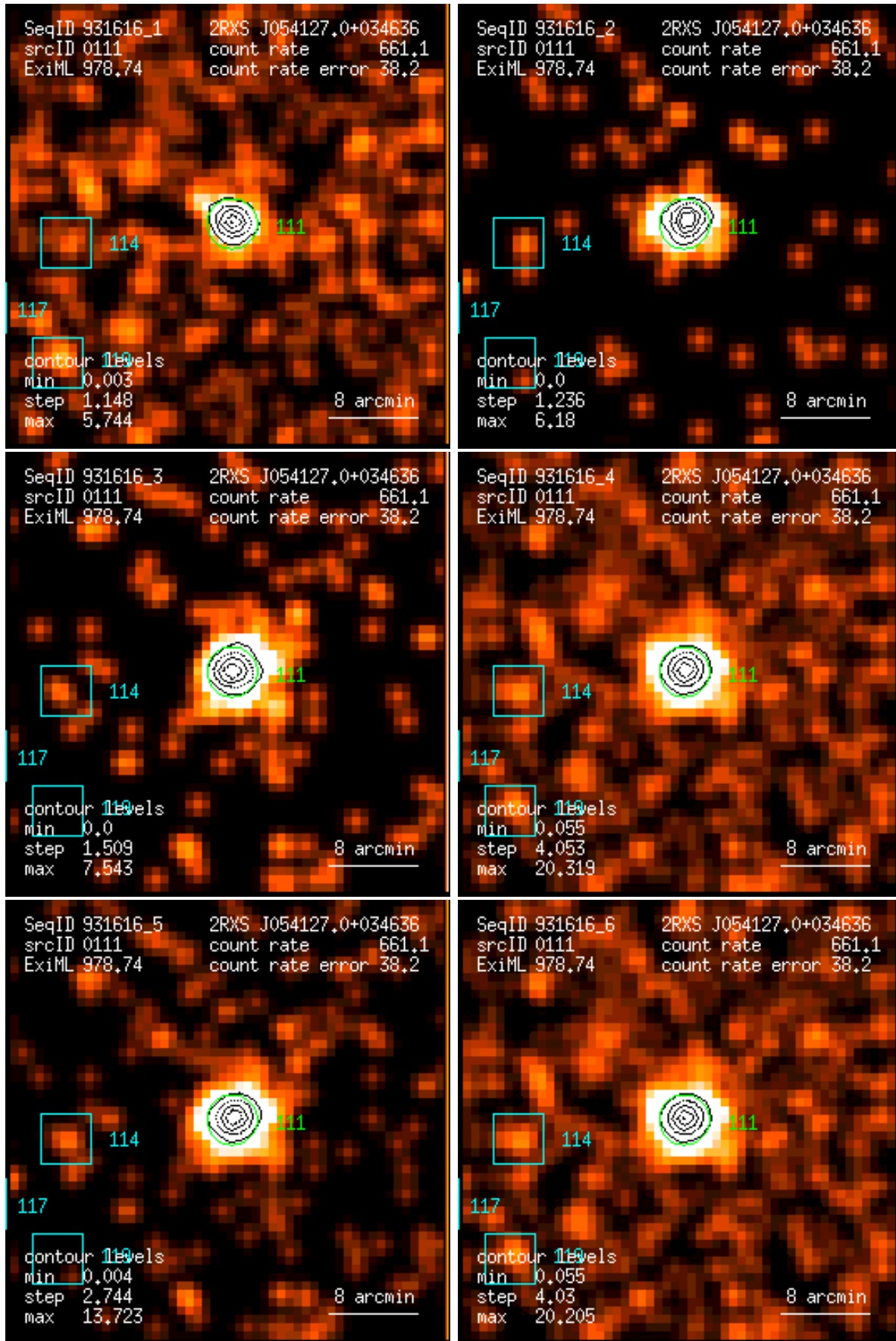
Figure 111: RASS 931616: detection 0111: band rate images, Gaussian filter: (1) PSPC channels 11 – 41, (2) 52 – 90, (3) 91 – 201, (4) 11 – 235, (5) 52 – 201, (6) 11 – 201. Broad band rates in counts/ks. Band rate contour levels in counts/ks/arcmin 2 .
