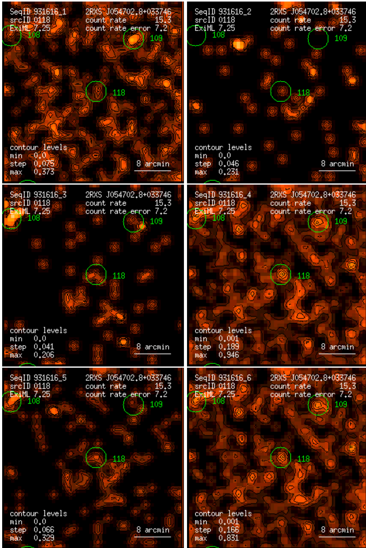
Figure 118: RASS 931616: detection 0118: band rate images, Gaussian filter: (1) PSPC channels 11 – 41, (2) 52 – 90, (3) 91 – 201, (4) 11 – 235, (5) 52 – 201, (6) 11 – 201. Broad band rates in counts/ks. Band rate contour levels in counts/ks/arcmin 2 .
