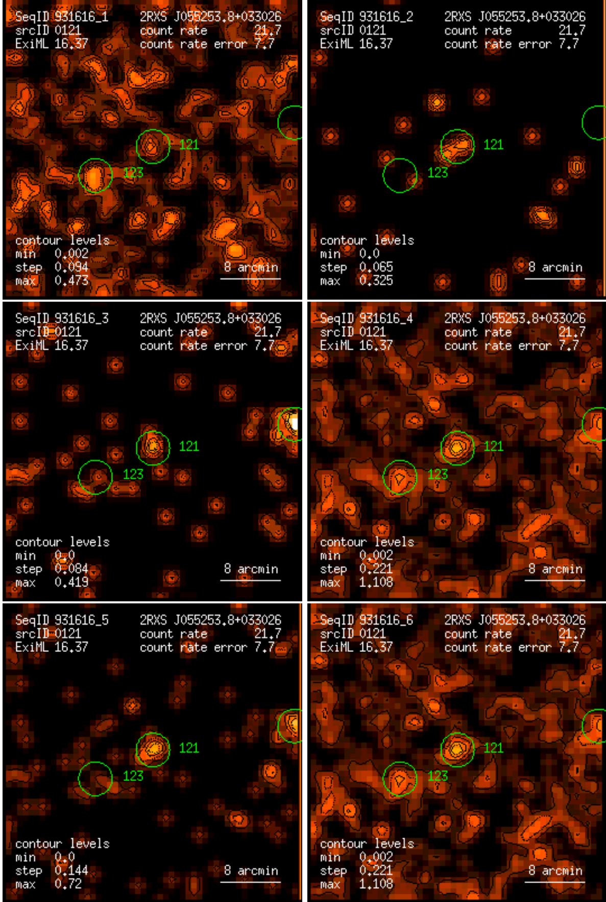
Figure 121: RASS 931616: detection 0121: band rate images, Gaussian filter: (1) PSPC channels 11 – 41, (2) 52 – 90, (3) 91 – 201, (4) 11 – 235, (5) 52 – 201, (6) 11 – 201. Broad band rates in counts/ks. Band rate contour levels in counts/ks/arcmin 2 .
