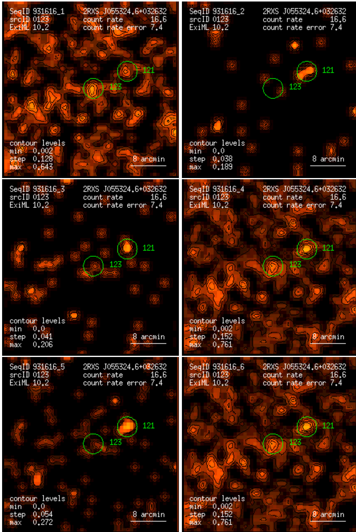
Figure 123: RASS 931616: detection 0123: band rate images, Gaussian filter: (1) PSPC channels 11 – 41, (2) 52 – 90, (3) 91 – 201, (4) 11 – 235, (5) 52 – 201, (6) 11 – 201. Broad band rates in counts/ks. Band rate contour levels in counts/ks/arcmin 2 .
