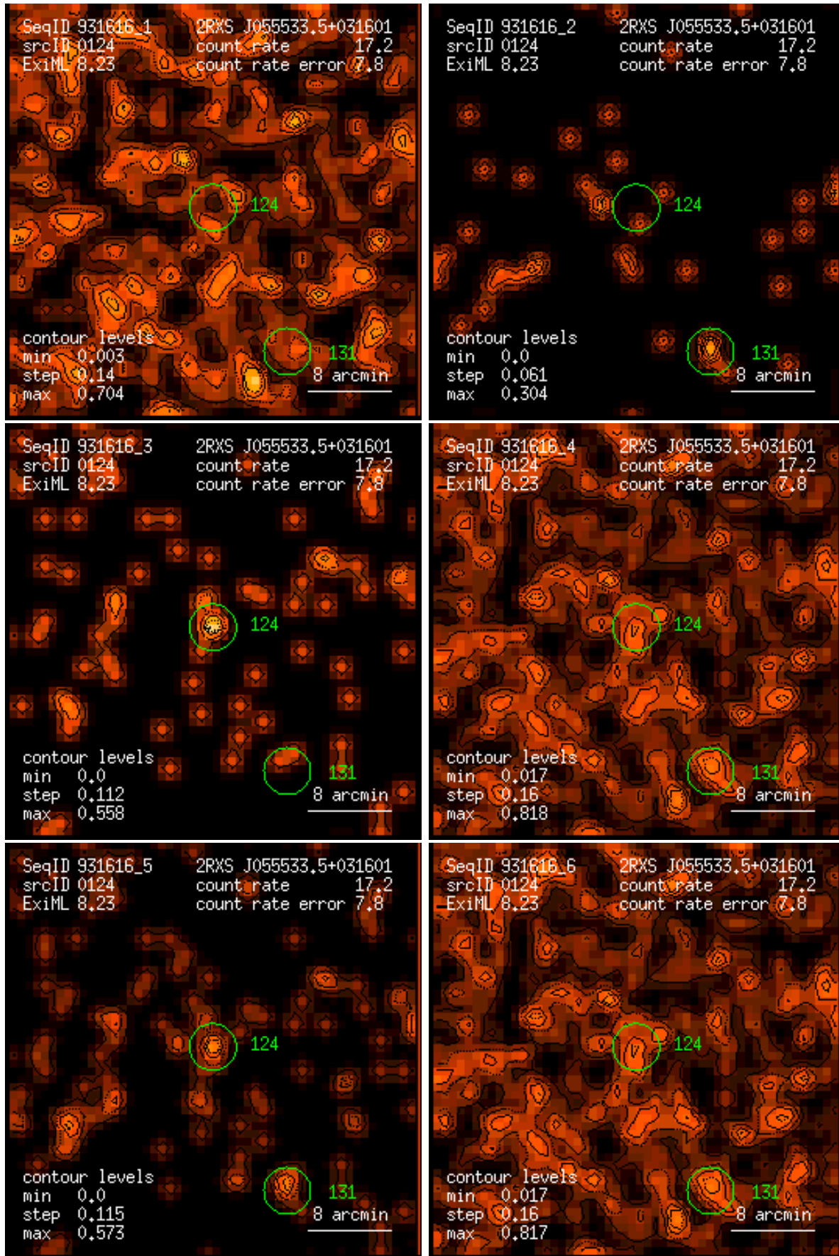
Figure 124: RASS 931616: detection 0124: band rate images, Gaussian filter: (1) PSPC channels 11 – 41, (2) 52 – 90, (3) 91 – 201, (4) 11 – 235, (5) 52 – 201, (6) 11 – 201. Broad band rates in counts/ks. Band rate contour levels in counts/ks/arcmin 2 .
