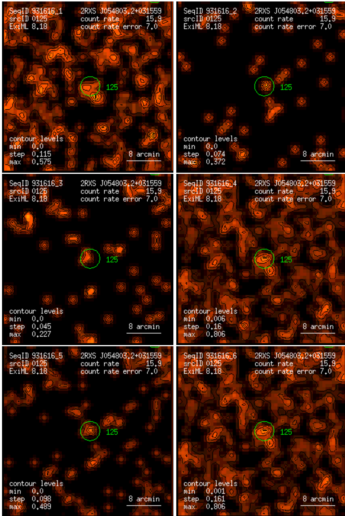
Figure 125: RASS 931616: detection 0125: band rate images, Gaussian filter: (1) PSPC channels 11 – 41, (2) 52 – 90, (3) 91 – 201, (4) 11 – 235, (5) 52 – 201, (6) 11 – 201. Broad band rates in counts/ks. Band rate contour levels in counts/ks/arcmin 2 .
