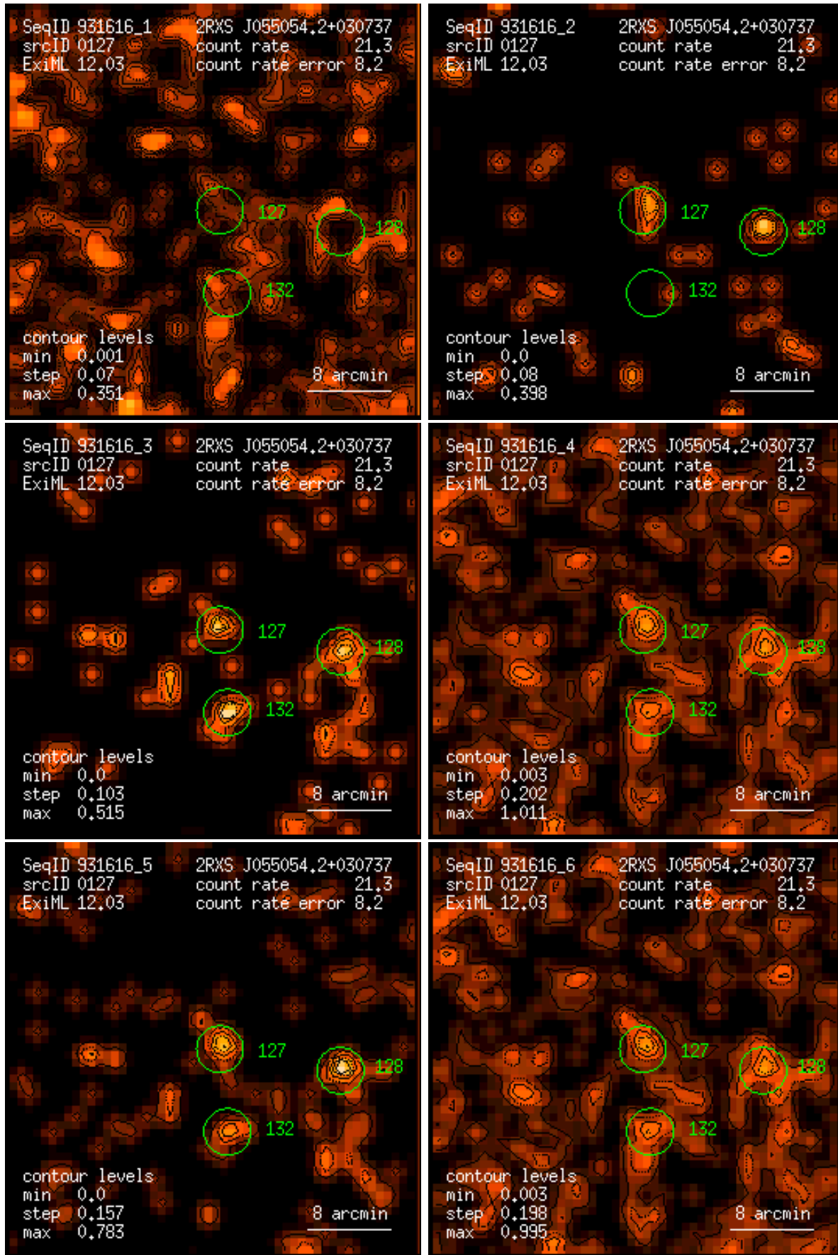
Figure 127: RASS 931616: detection 0127: band rate images, Gaussian filter: (1) PSPC channels 11 – 41, (2) 52 – 90, (3) 91 – 201, (4) 11 – 235, (5) 52 – 201, (6) 11 – 201. Broad band rates in counts/ks. Band rate contour levels in counts/ks/arcmin 2 .
