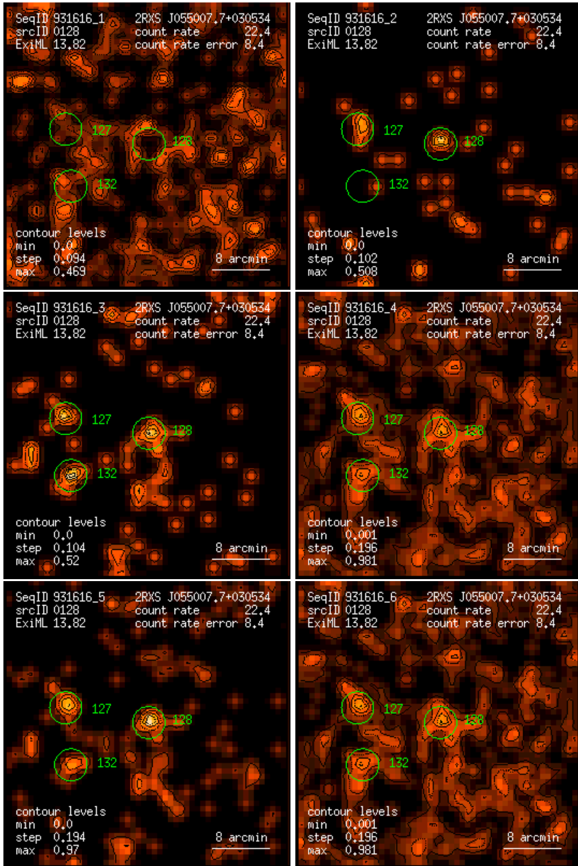
Figure 128: RASS 931616: detection 0128: band rate images, Gaussian filter: (1) PSPC channels 11 – 41, (2) 52 – 90, (3) 91 – 201, (4) 11 – 235, (5) 52 – 201, (6) 11 – 201. Broad band rates in counts/ks. Band rate contour levels in counts/ks/arcmin 2 .
