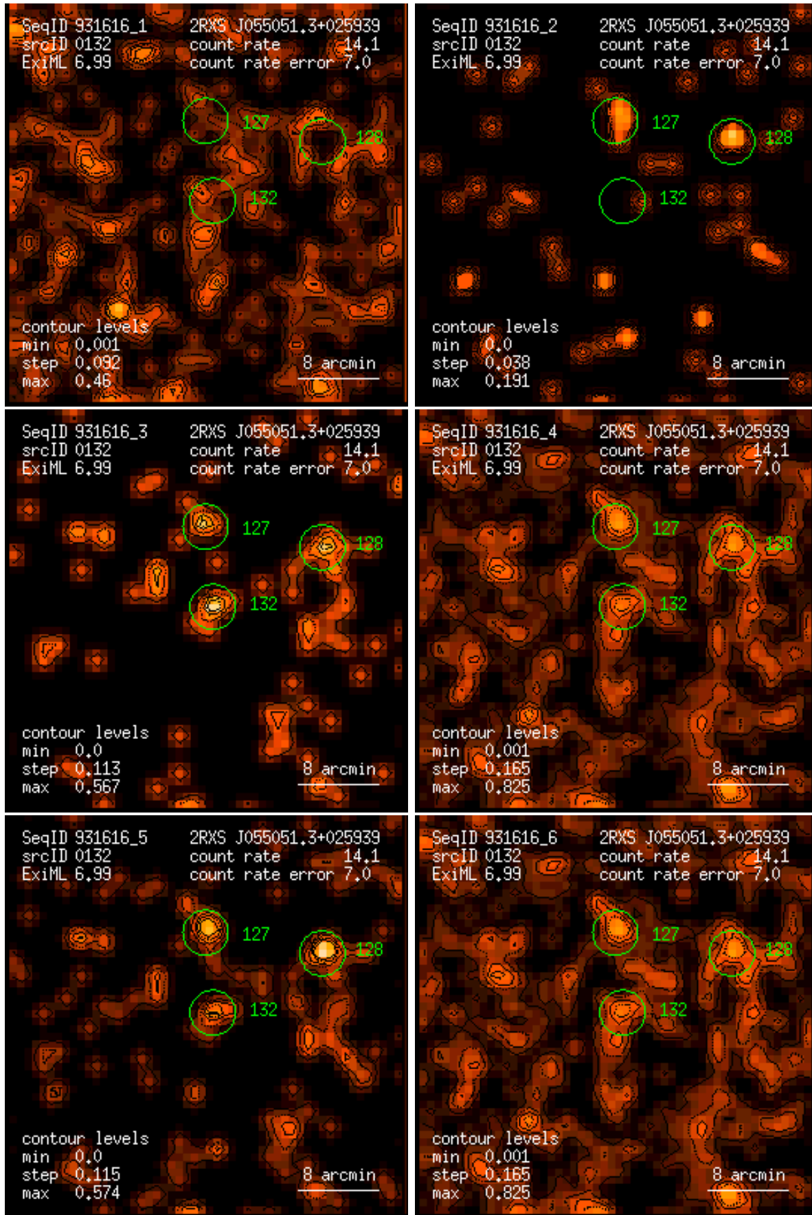
Figure 132: RASS 931616: detection 0132: band rate images, Gaussian filter: (1) PSPC channels 11 – 41, (2) 52 – 90, (3) 91 – 201, (4) 11 – 235, (5) 52 – 201, (6) 11 – 201. Broad band rates in counts/ks. Band rate contour levels in counts/ks/arcmin 2 .
