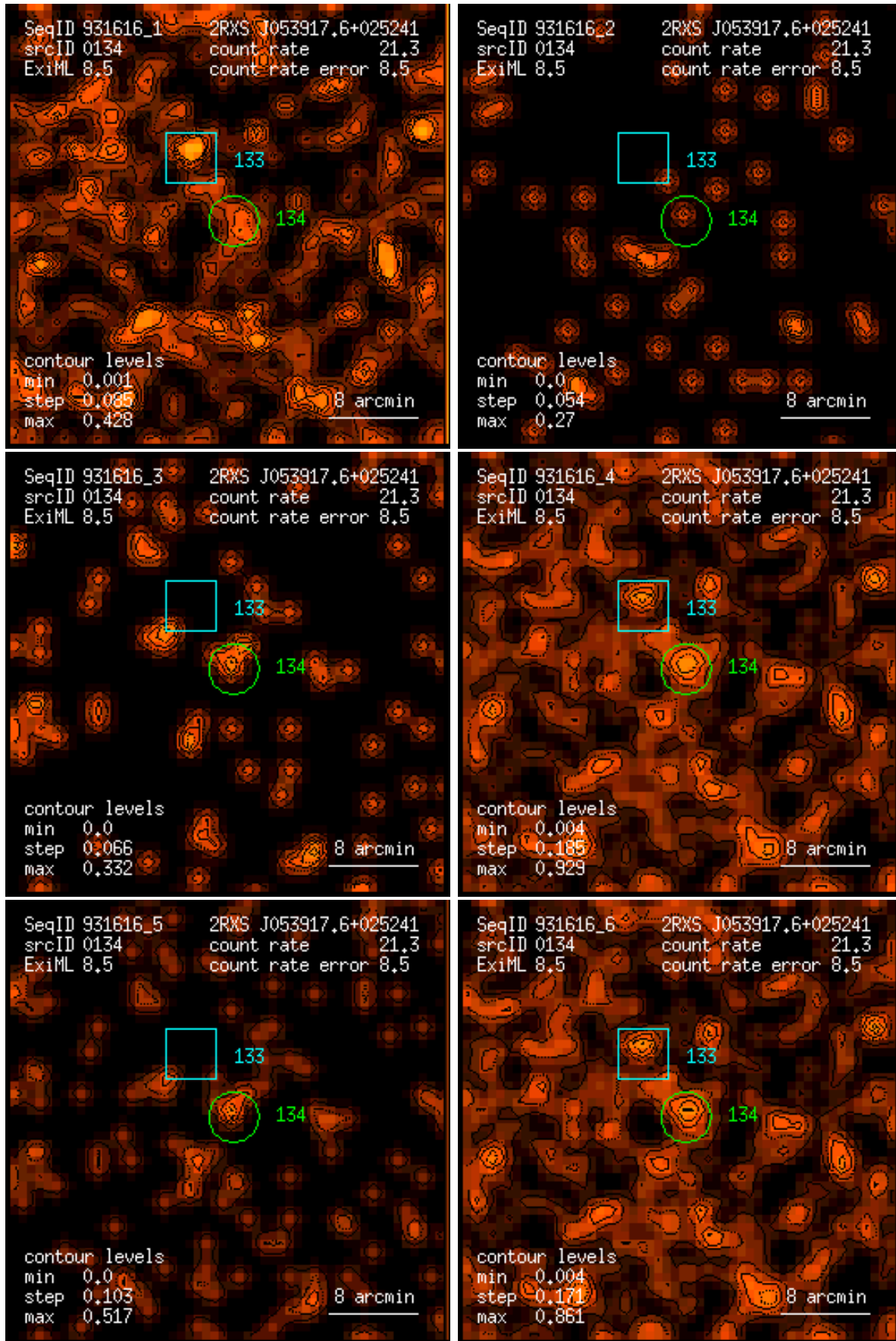
Figure 134: RASS 931616: detection 0134: band rate images, Gaussian filter: (1) PSPC channels 11 – 41, (2) 52 – 90, (3) 91 – 201, (4) 11 – 235, (5) 52 – 201, (6) 11 – 201. Broad band rates in counts/ks. Band rate contour levels in counts/ks/arcmin 2 .
