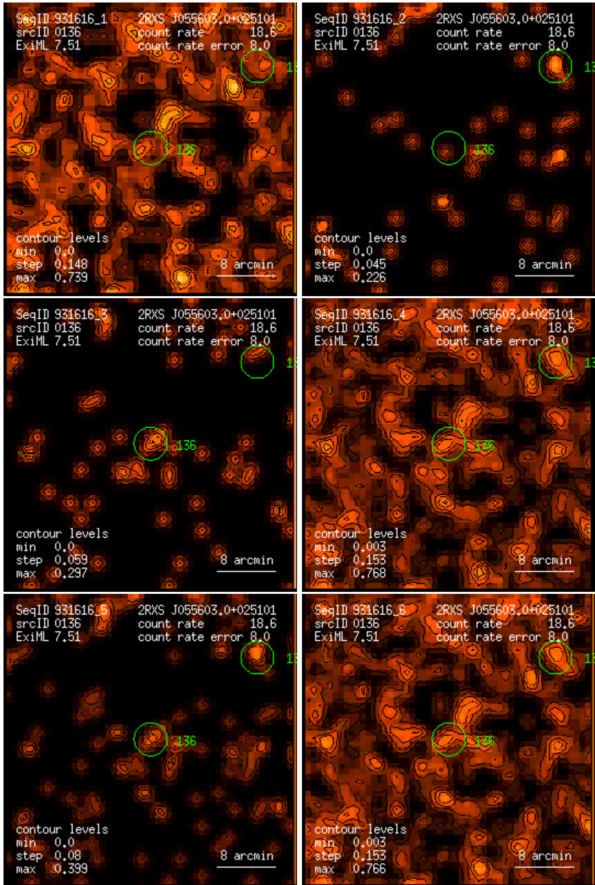
Figure 136: RASS 931616: detection 0136: band rate images, Gaussian filter: (1) PSPC channels 11 – 41, (2) 52 – 90, (3) 91 – 201, (4) 11 – 235, (5) 52 – 201, (6) 11 – 201. Broad band rates in counts/ks. Band rate contour levels in counts/ks/arcmin 2 .
