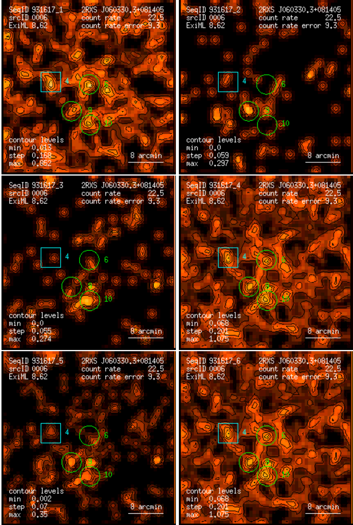
Figure 6: RASS 931617: detection 0006: band rate images, Gaussian filter: (1) PSPC channels 11 – 41, (2) 52 – 90, (3) 91 – 201, (4) 11 – 235, (5) 52 – 201, (6) 11 – 201. Broad band rates in counts/ks. Band rate contour levels in counts/ks/arcmin 2 .
