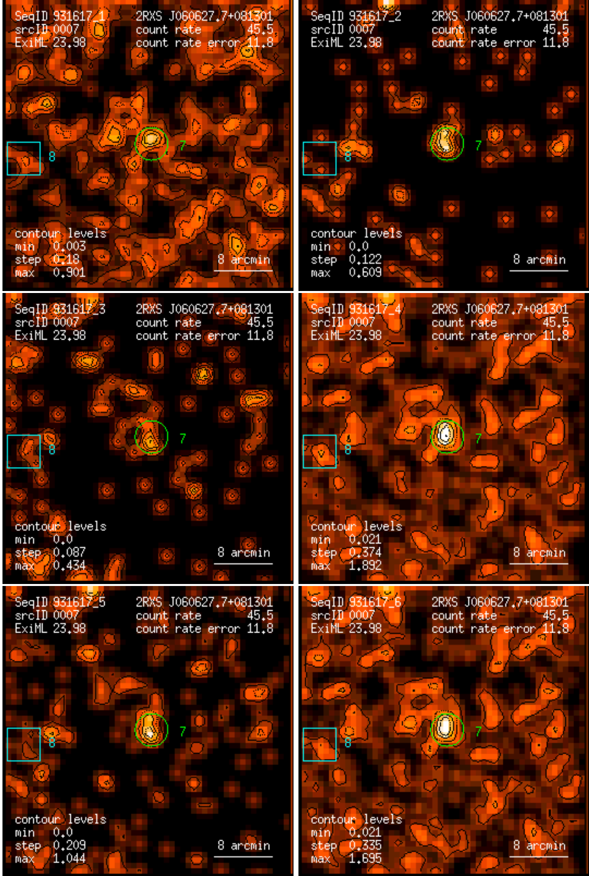
Figure 7: RASS 931617: detection 0007: band rate images, Gaussian filter: (1) PSPC channels 11 – 41, (2) 52 – 90, (3) 91 – 201, (4) 11 – 235, (5) 52 – 201, (6) 11 – 201. Broad band rates in counts/ks. Band rate contour levels in counts/ks/arcmin 2 .
