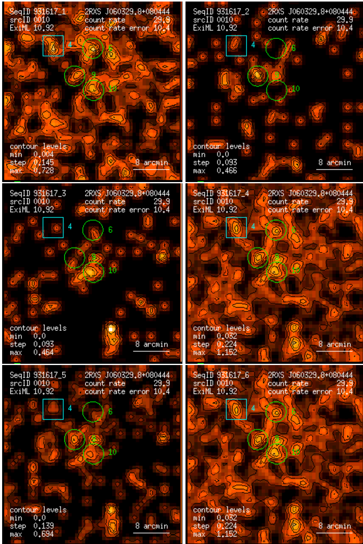
Figure 10: RASS 931617: detection 0010: band rate images, Gaussian filter: (1) PSPC channels 11 – 41, (2) 52 – 90, (3) 91 – 201, (4) 11 – 235, (5) 52 – 201, (6) 11 – 201. Broad band rates in counts/ks. Band rate contour levels in counts/ks/arcmin 2 .
