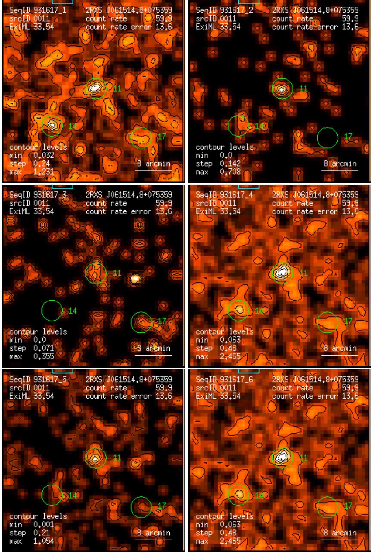
Figure 11: RASS 931617: detection 0011: band rate images, Gaussian filter: (1) PSPC channels 11 – 41, (2) 52 – 90, (3) 91 – 201, (4) 11 – 235, (5) 52 – 201, (6) 11 – 201. Broad band rates in counts/ks. Band rate contour levels in counts/ks/arcmin 2 .
